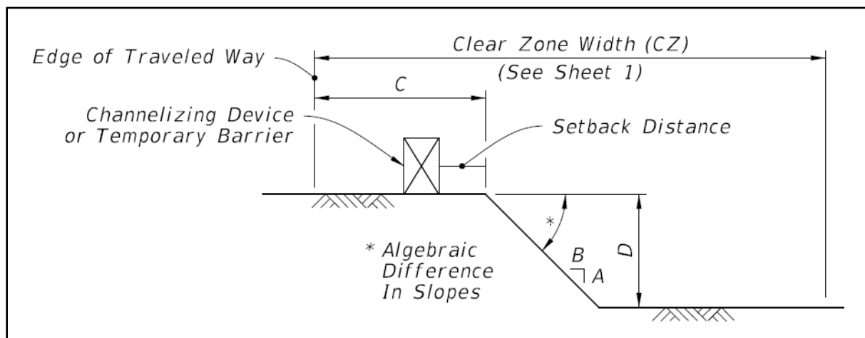
Figure 4 – 10 Drop-Off Condition Detail
