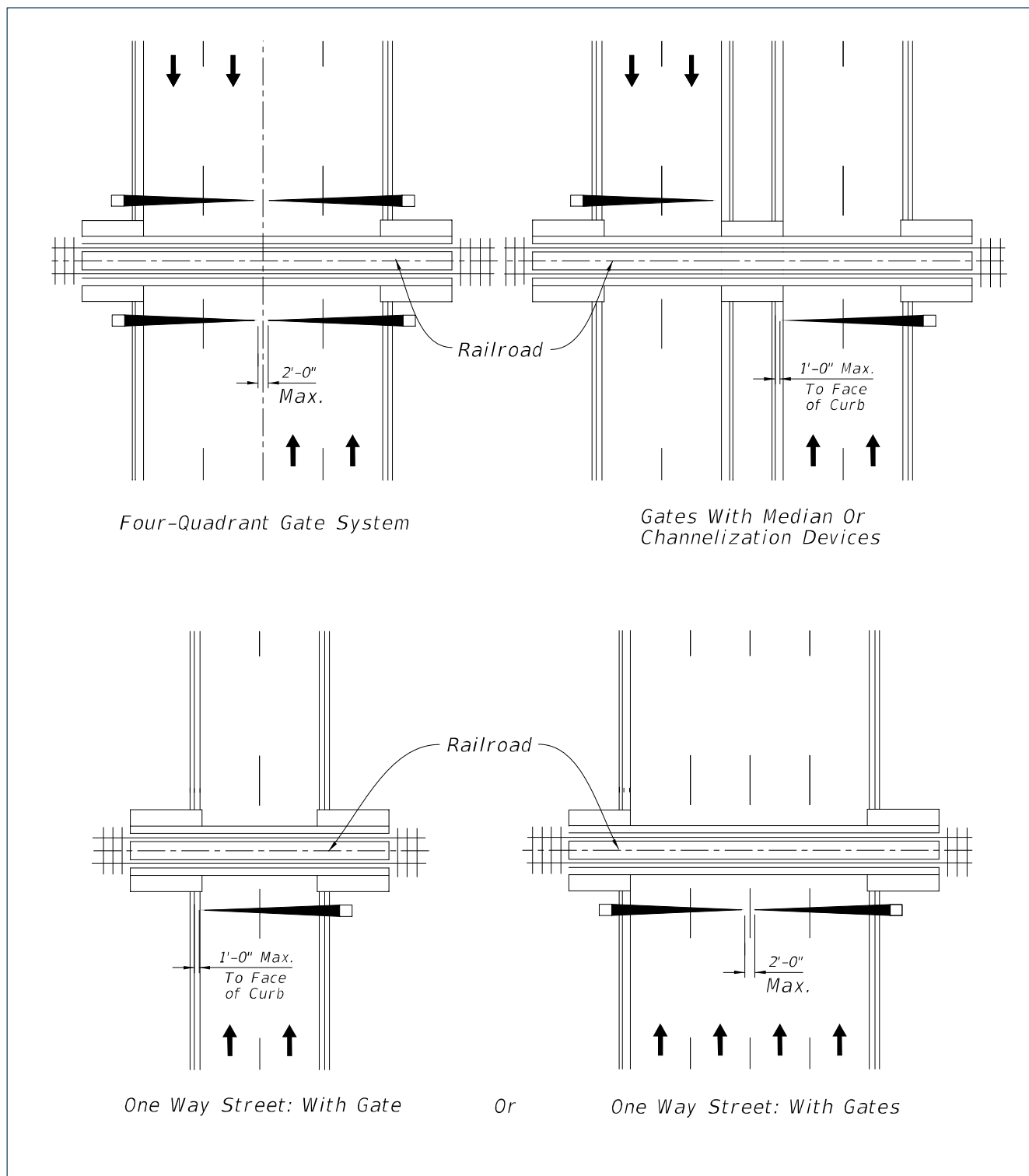
Figure 85-1 Gate Configuration for Quiet Zones
