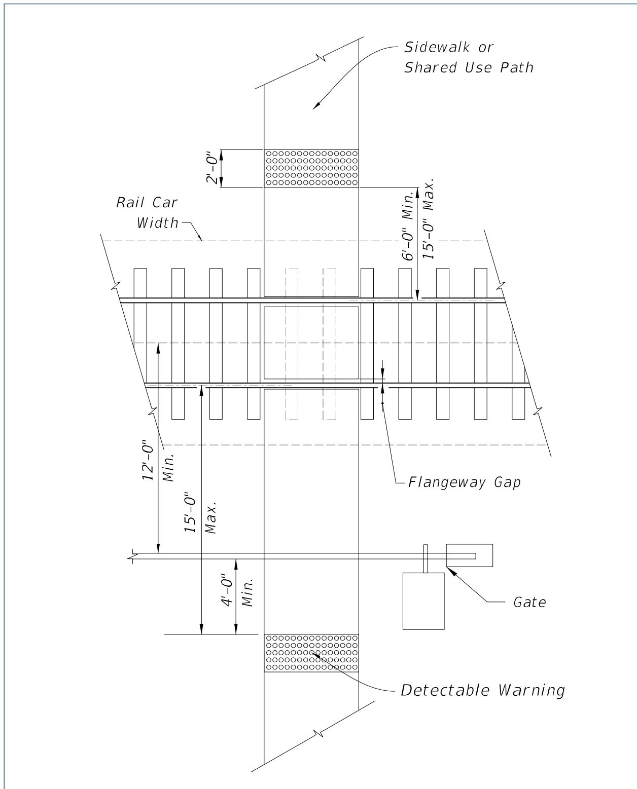
Figure 7-3 Pedestrian Crossings
