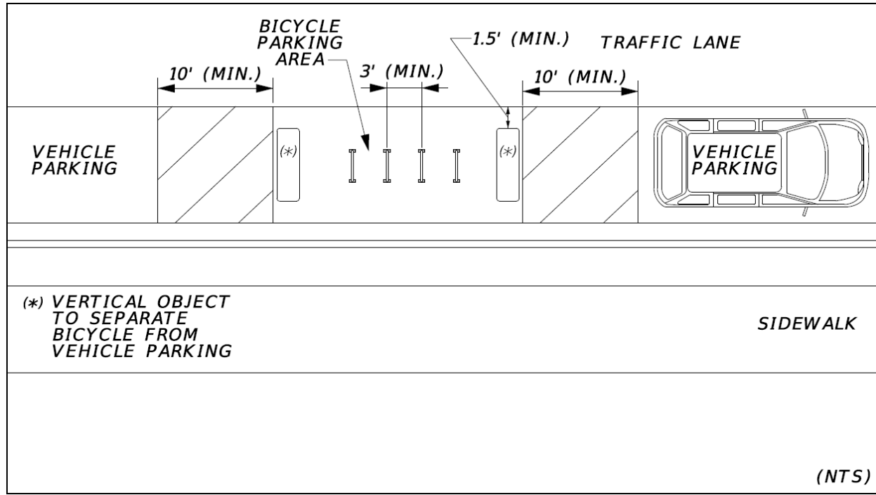
Figure 223.5.1 On-Street Bicycle Parking (Midblock)
