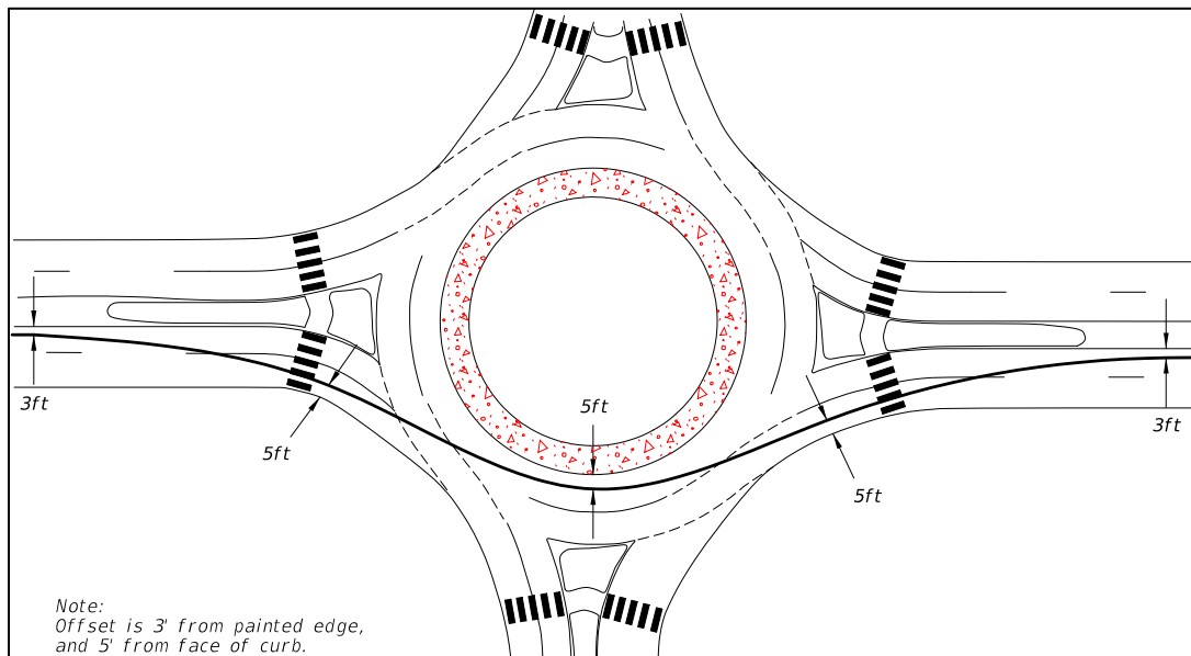
Figure 213.6.42 Fastest Path for Through Movement
