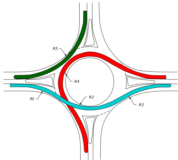
Figure 213.6.1 Fastest Path Curves
