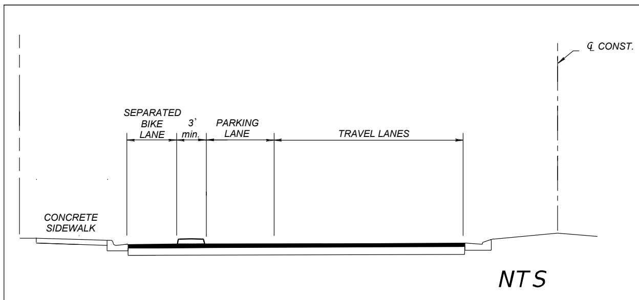
Figure 223.2.23 On-Street Parking Minimal Separation
