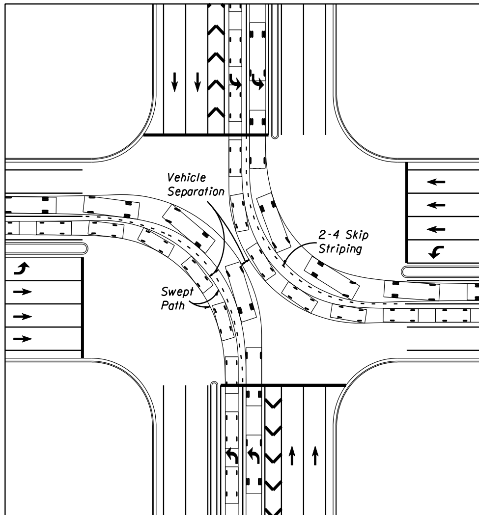
Figure 212.12.56 P and SU Design Vehicles Turning Simultaneously
