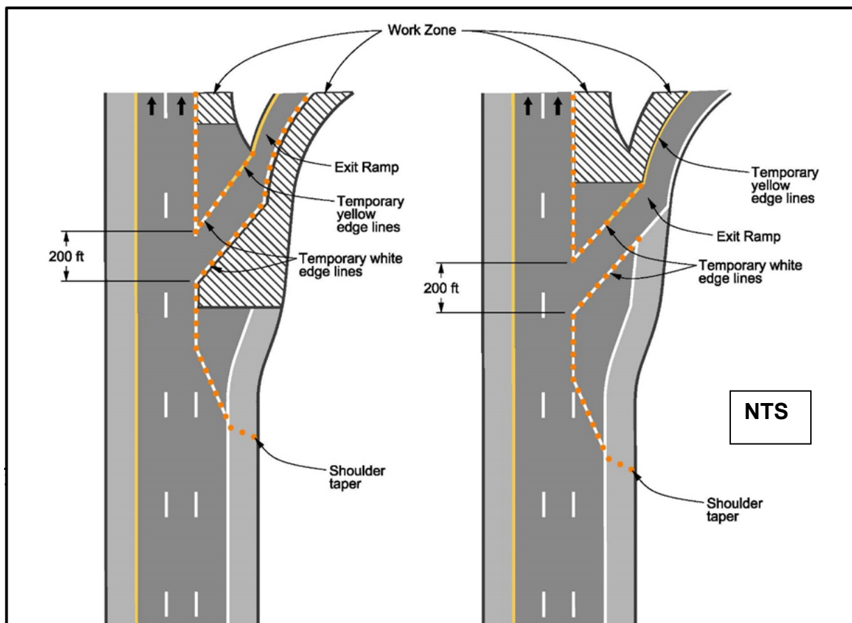
Figure 240.2.1 Work in the Vicinity of an Exit Ramp
