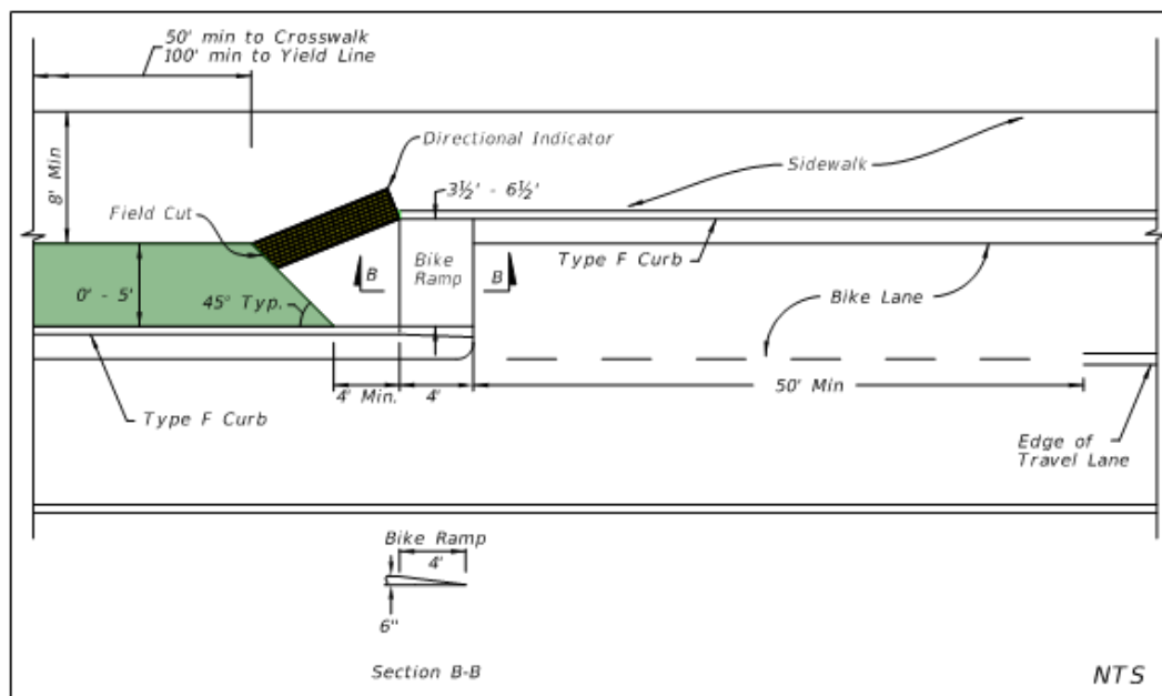
Figure 223.2.6 Straight Bicycle Ramp
