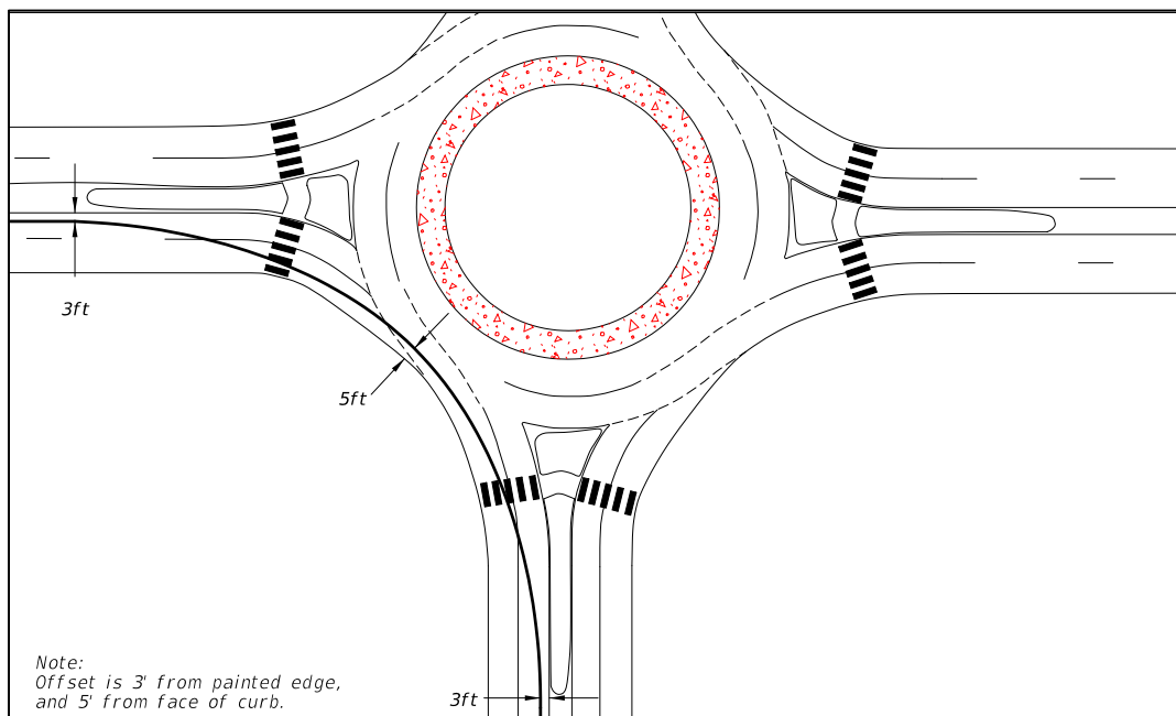
Figure 213.6.23 Fastest Path for Right Turn Movement
