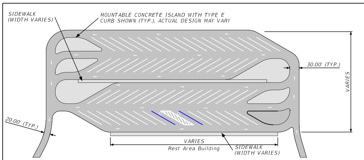
Figure 227.7.2: Multiple Bay Pull-Through
