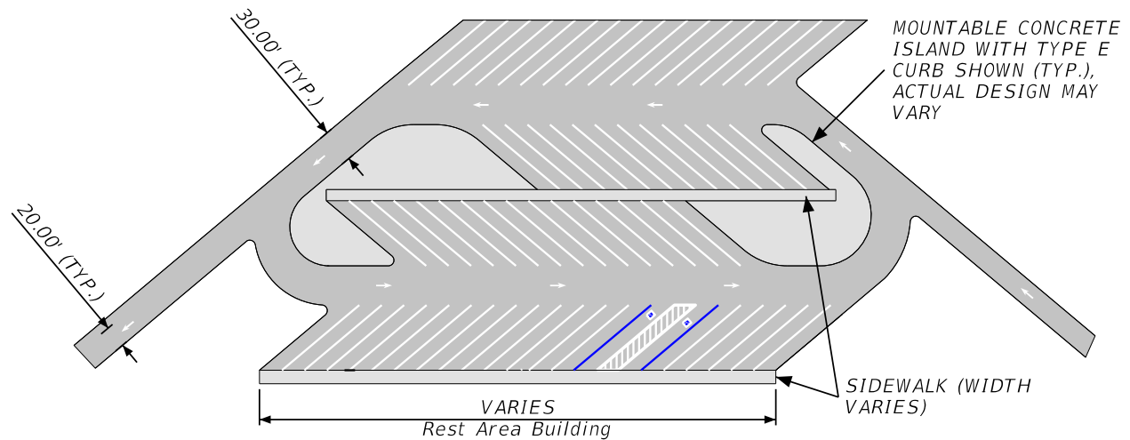
Figure 227.7.6: Parking Stall Angled Back-In
