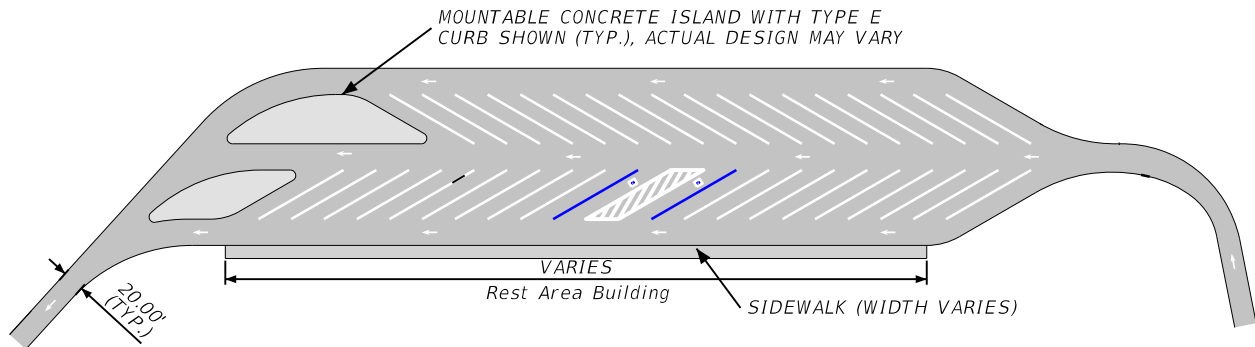
Figure 227.7.2: Multiple Bay Pull-Through
