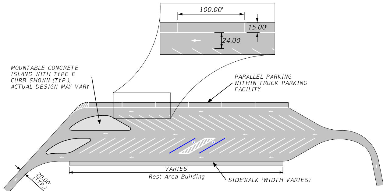
Figure 227.7.8-7: Parallel Parking within Truck Parking Facility
