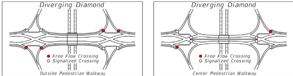
Figure 217.6.1 Pedestrian Routing Methods
