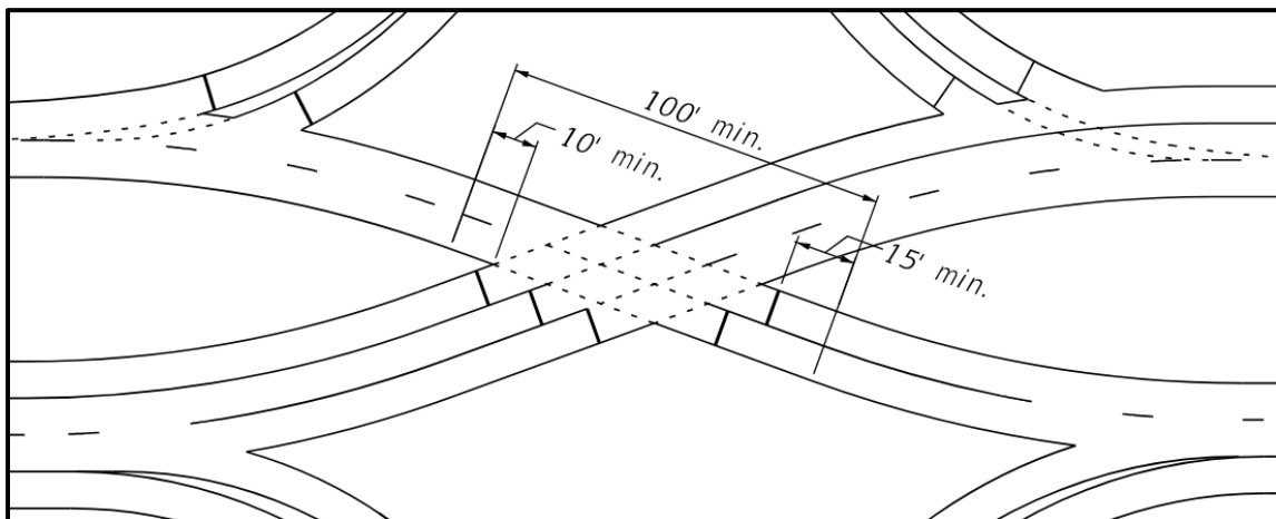
Figure 217.3.3 Tangents at Crossover Intersections
