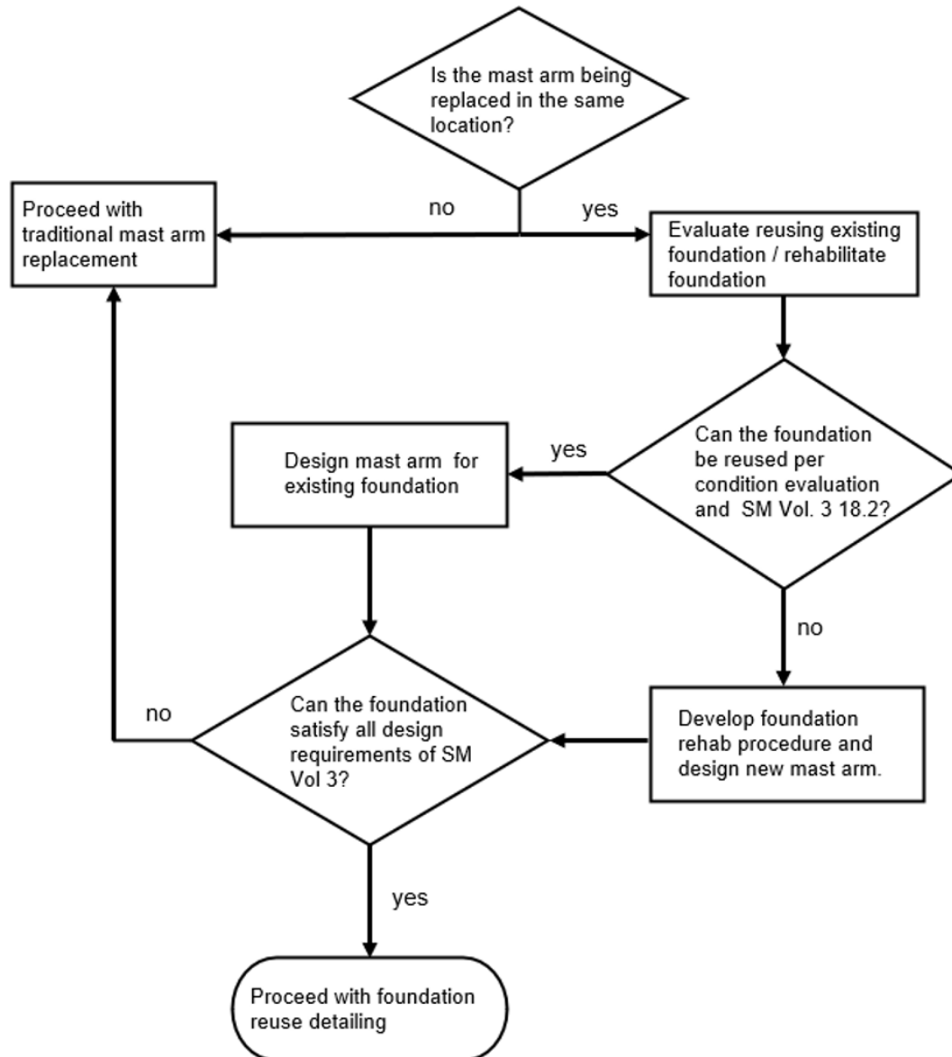
Figure 261.8.1 Flowchart for Determining Foundation Reuse
