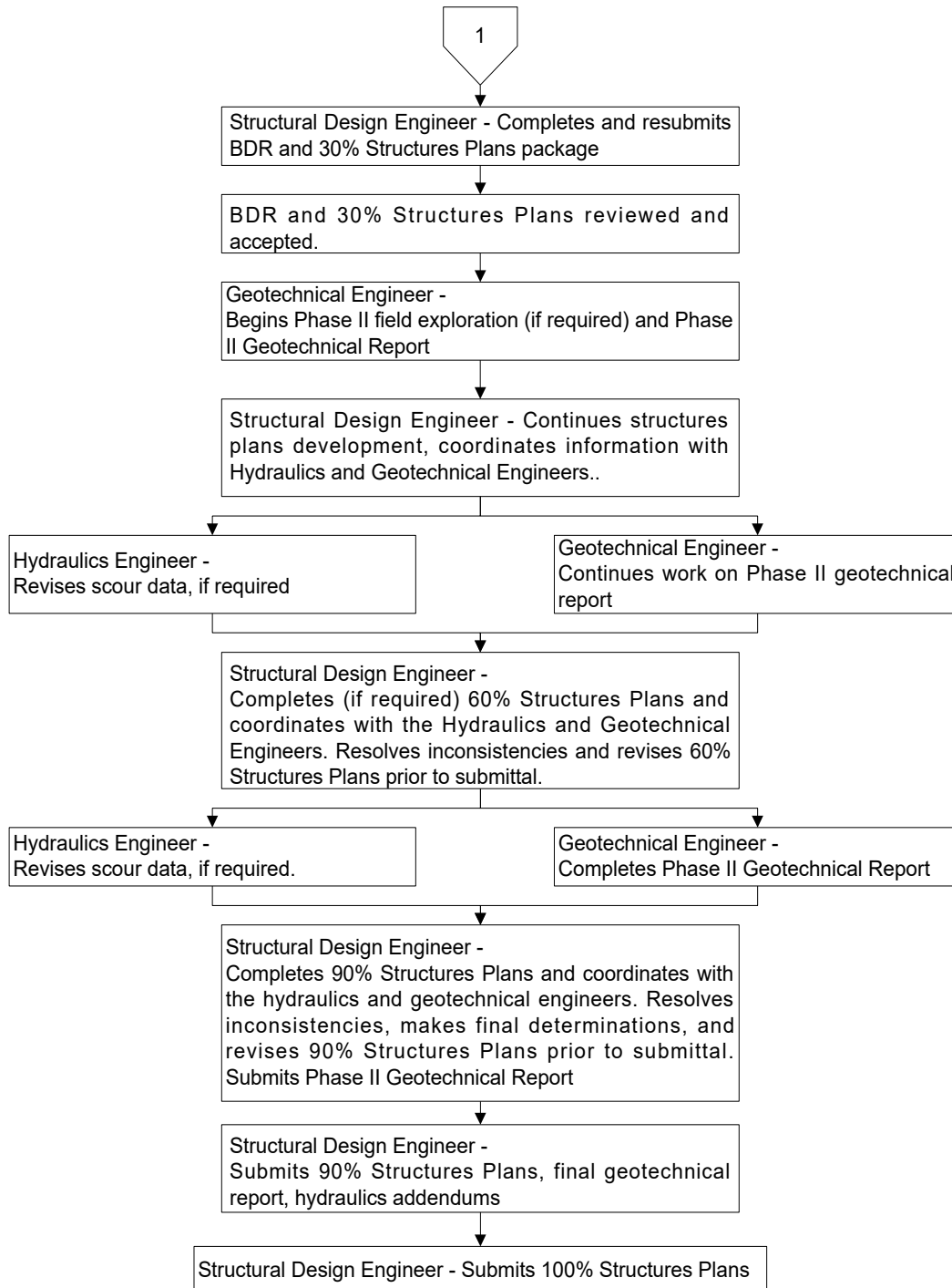
Figure 250.2.1 Structural Plans Development Sheet 2 of 2
