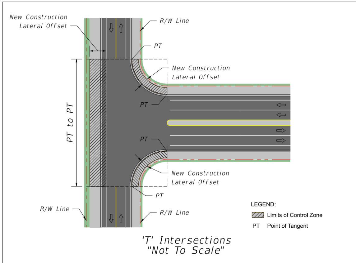
Figure 215.2.5 'T' Intersection
