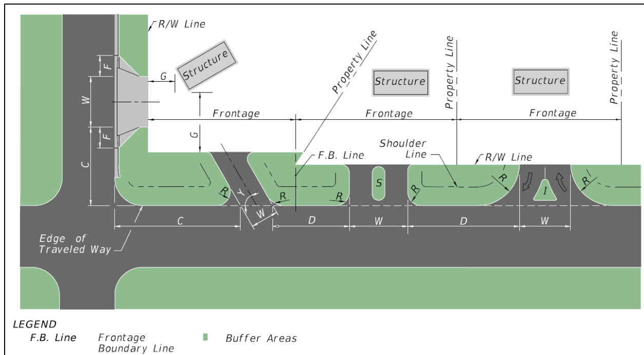
Figure 214.1.1 Driveway Terminology
