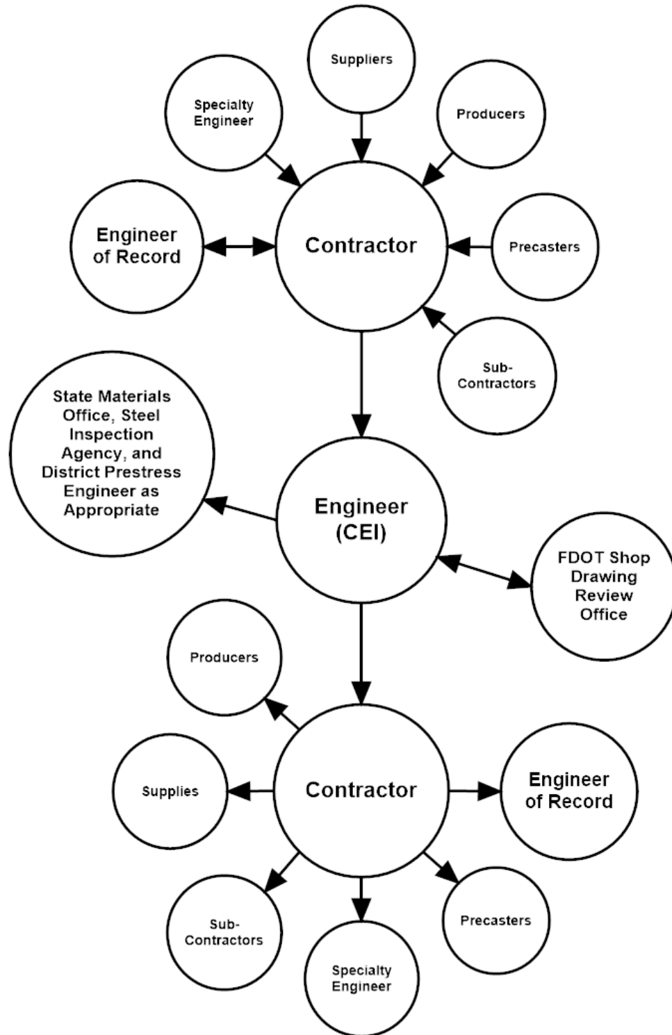
Figure 152.11.5 Shop Drawing Flow Diagram for Design-Build Projects-Shop Drawings Not Affecting Public Safety
