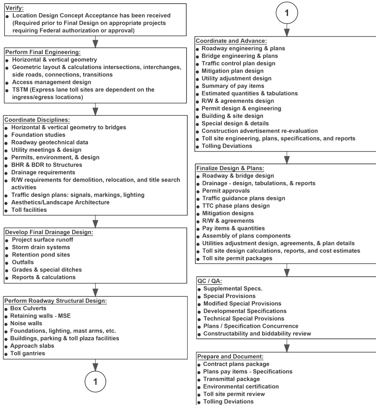
Figure 111.1.1 Major Activities – Final Engineering Design Process
