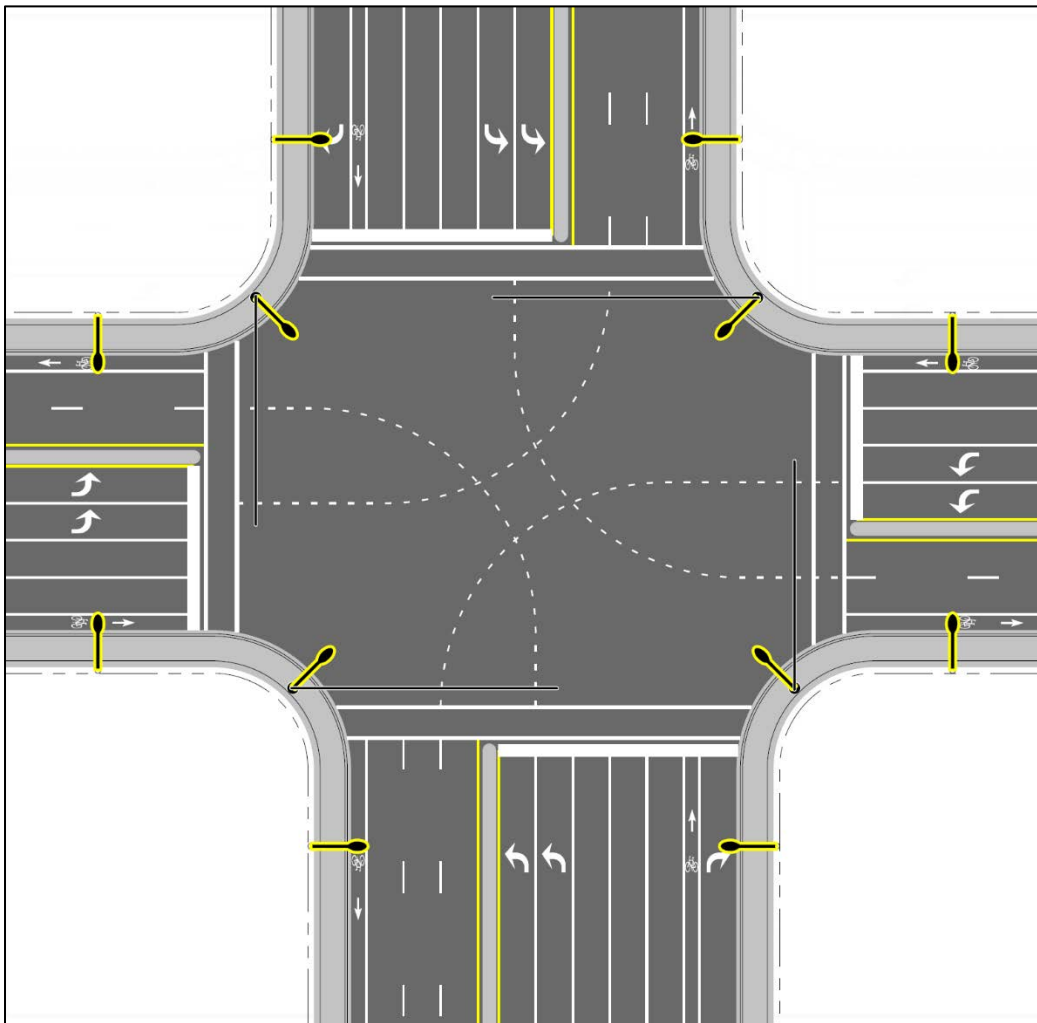
Figure 231.3.4 Typical Lighting Layout for Large Intersection
