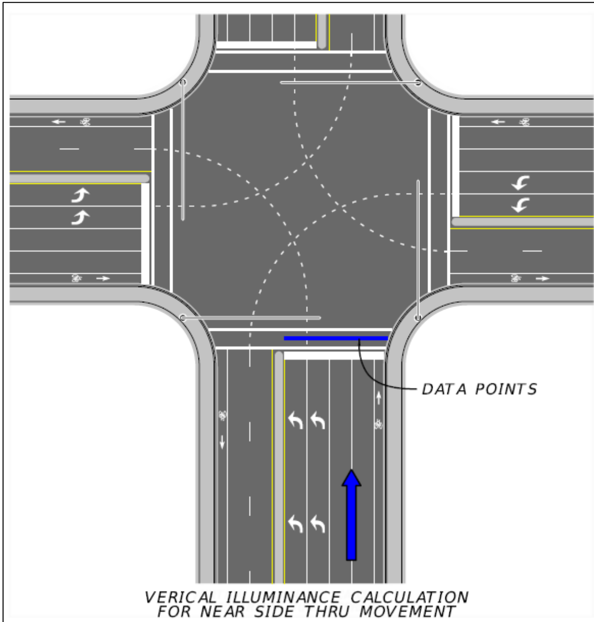
Figure 231.3.1 Vertical Illuminance Calculation for Near Side Movement
