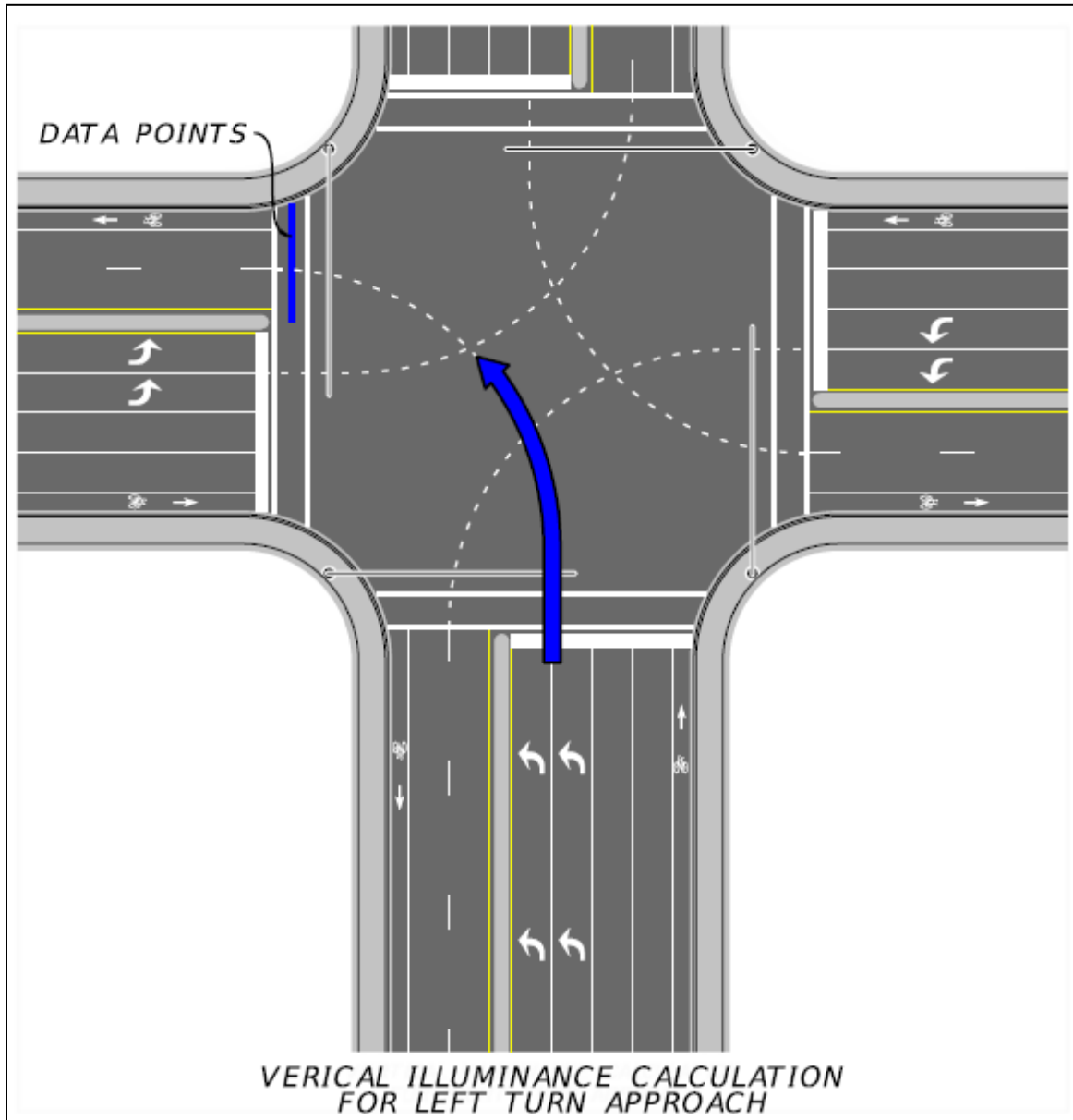
Figure 231.3.3 Vertical Illuminance Calculation for Left-Turn Approach
