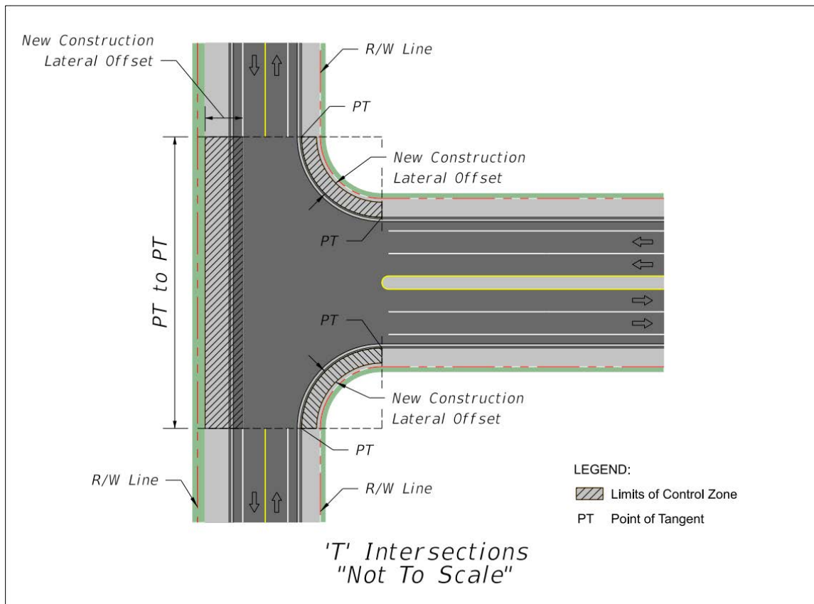
Figure 215.2.5 'T' Intersection
