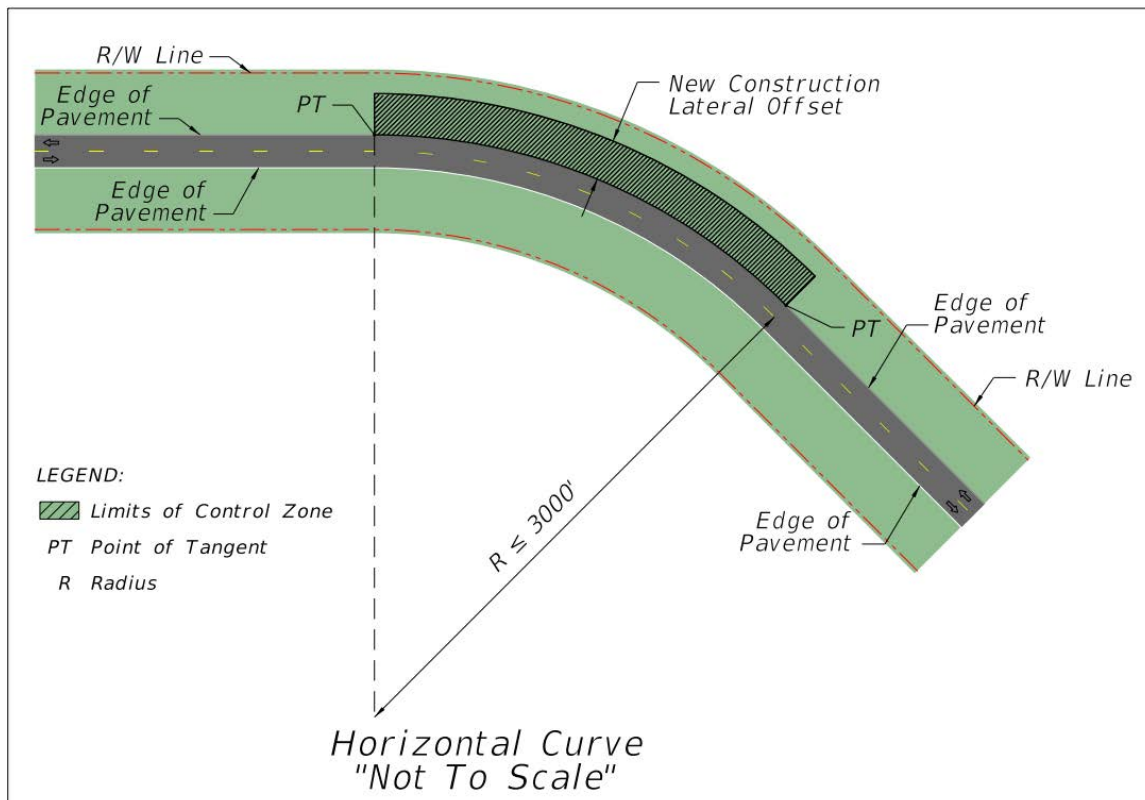
Figure 215.2.12 Horizontal Curve
