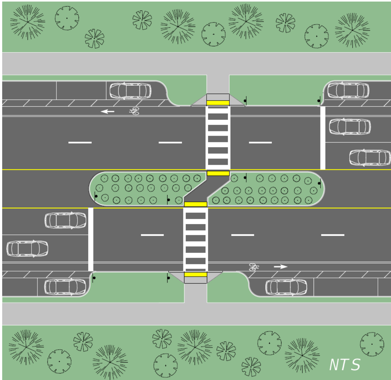
Figure 210.3.4 Midblock Refuge Island Example #1
