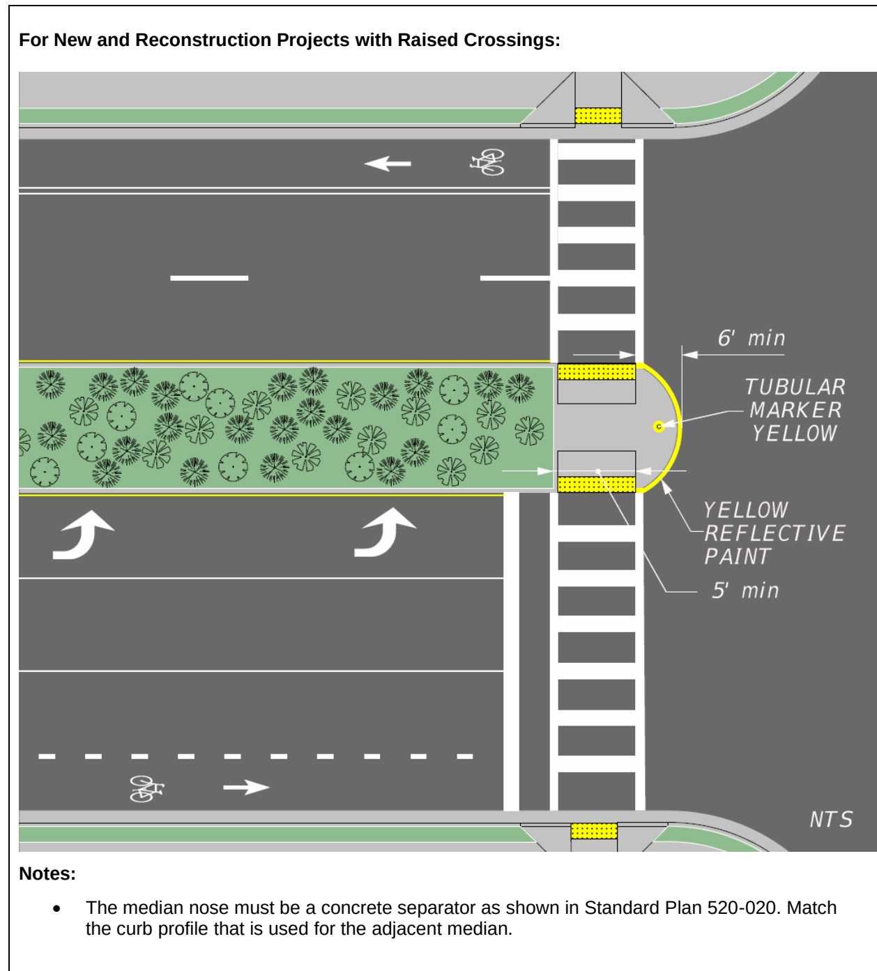
Figure 210.3.3 Intersection Refuge Island
