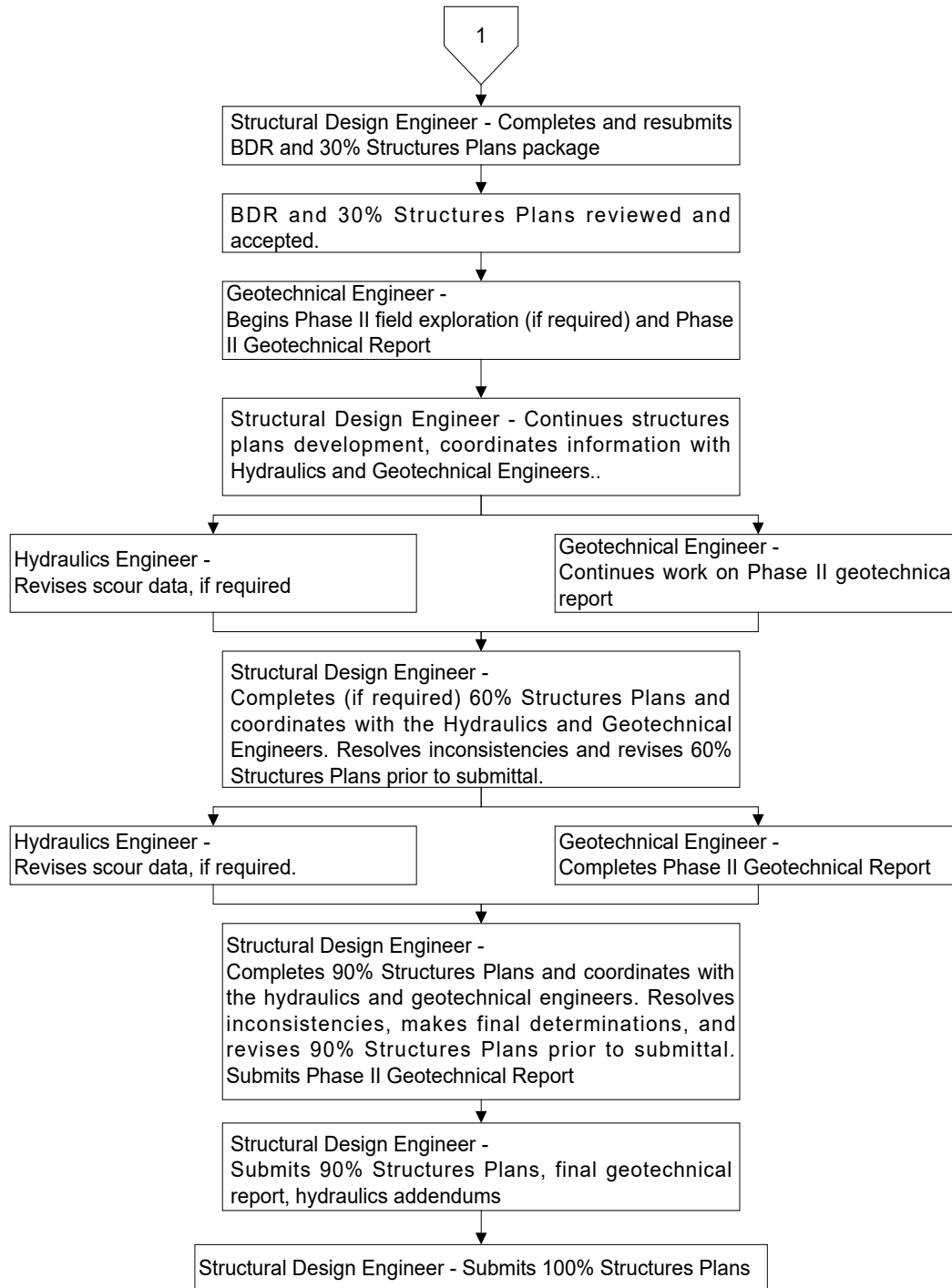
Figure 250.2.1 Structural Plans Development
