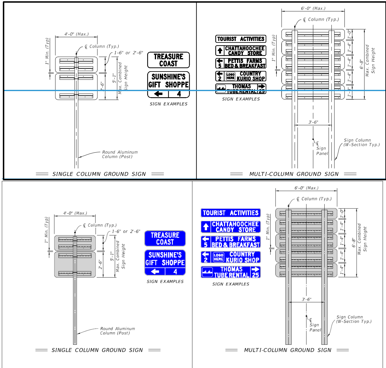
Figure 230.2.1 Tourist-Oriented Directional Sign Panel Dimensions
