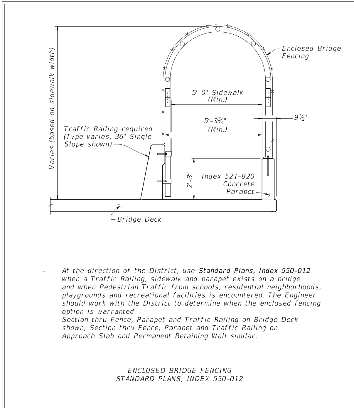
Figure 222.4.8 Bridge Railing – Enclosed Fencing
