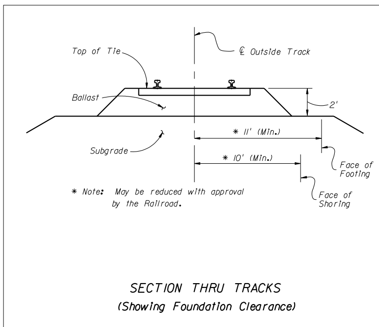
Figure 220.3.2 Section Through Tracks
