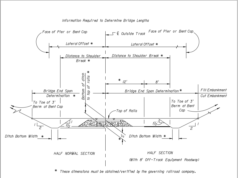
Figure 220.3.1 Track Section
