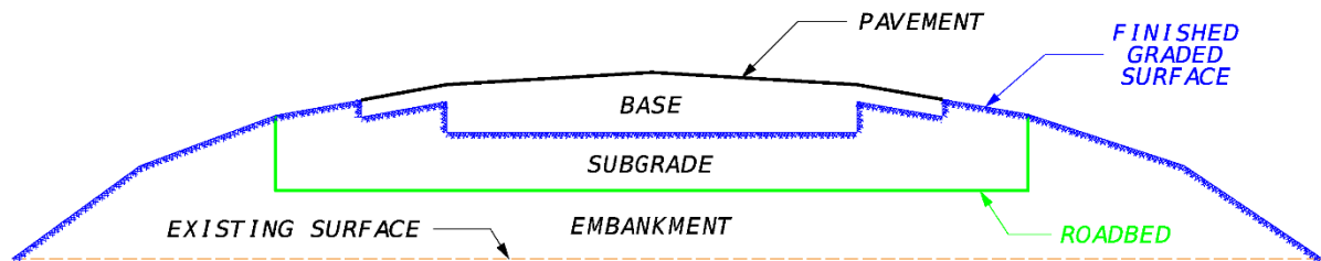
Figure 216.4.1 Finished Graded Surface
