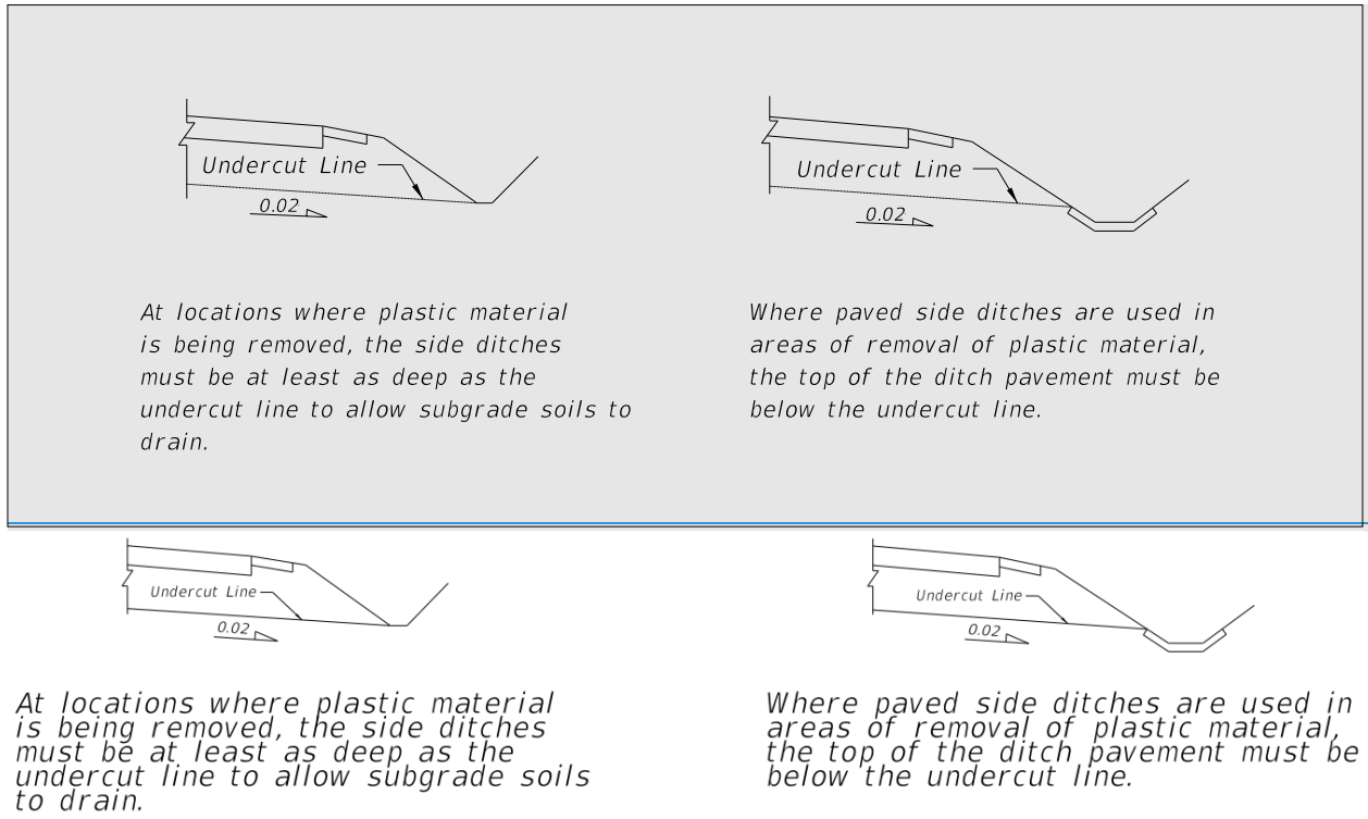
Figure 216.4.7 Undercut Detail of Plastic Material with Relation to Side Ditches
