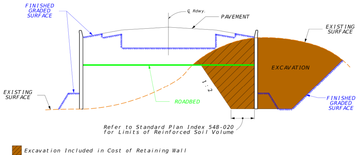
Figure 216.4.9 Retaining Wall Excavation and Embankment
