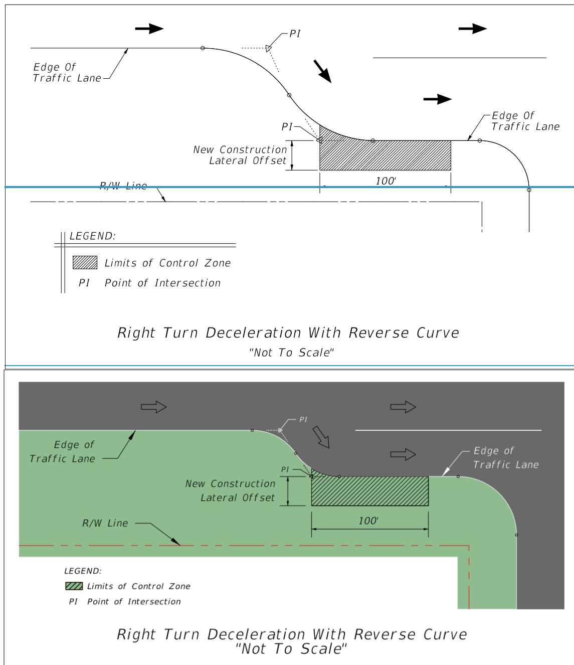
Figure 215.2.7 Right-Turn Deceleration with Reverse Curve
