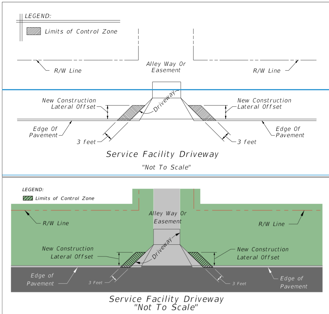
Figure 215.2.10 Service Facility Driveway
