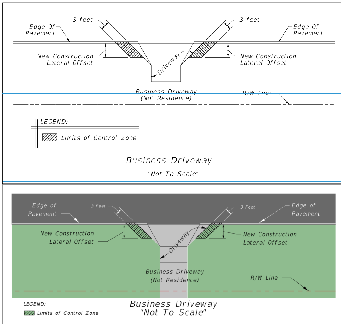
Figure 215.2.11 Business Driveway
