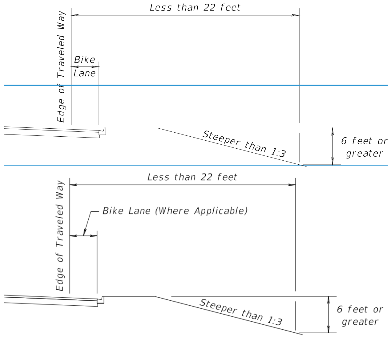
Figure 215.3.3 Drop-off Hazard on Low-Speed Curbed Roadways
