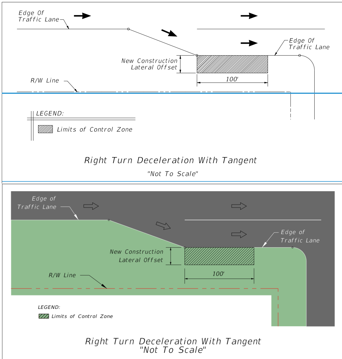
Figure 215.2.6 Right-Turn Deceleration with Tangent
