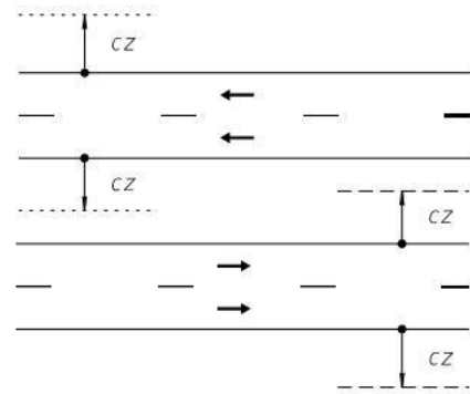
MULTI-LANE
