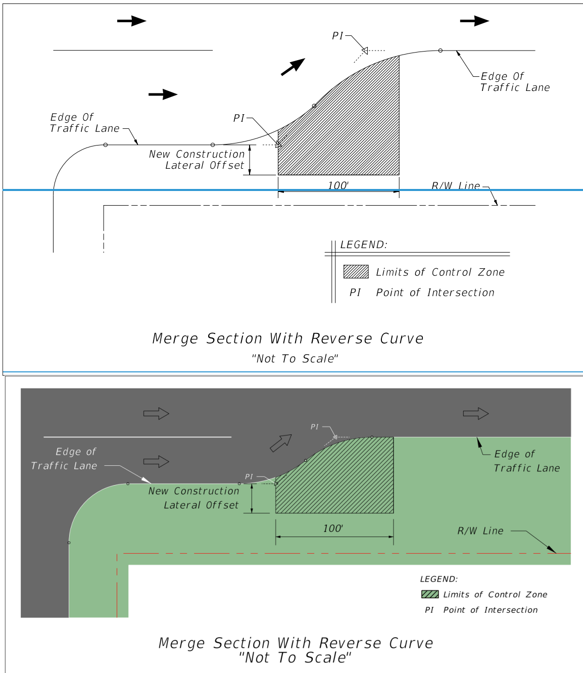
Figure 215.2.9 Merge Section with Reverse Curve
