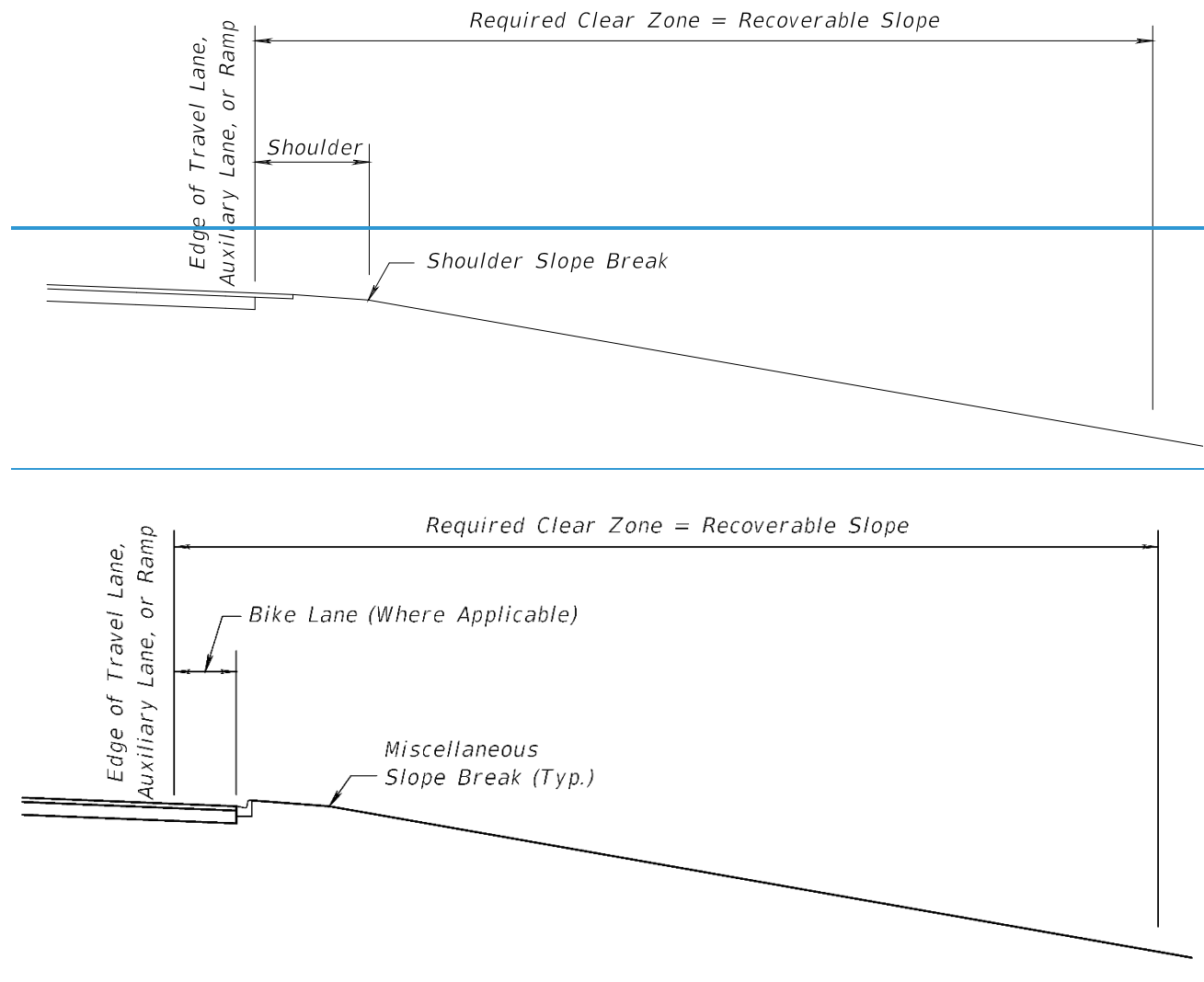
Figure 215.2.2 Clear Zone Concept
