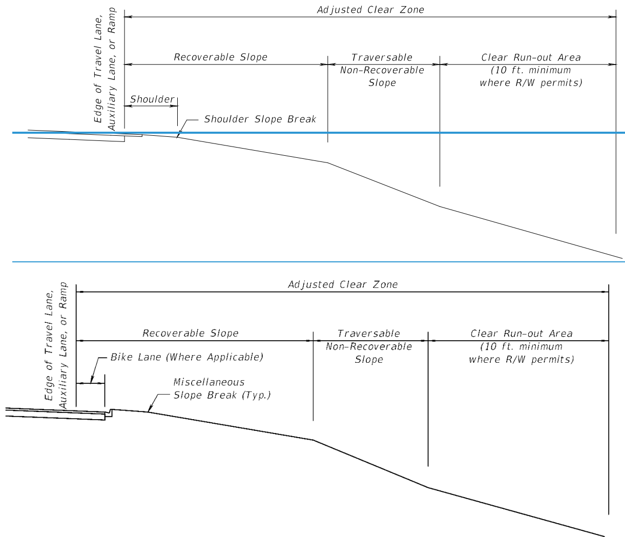
Figure 215.2.3 Adjusted Clear Zone Concept
