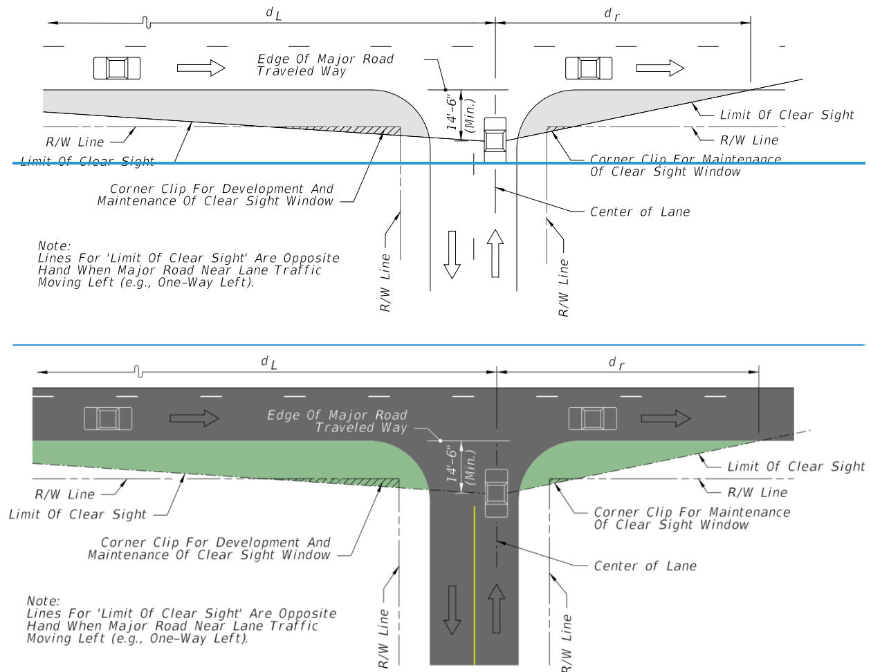
Figure 212.11.1 Clear Sight Triangles
