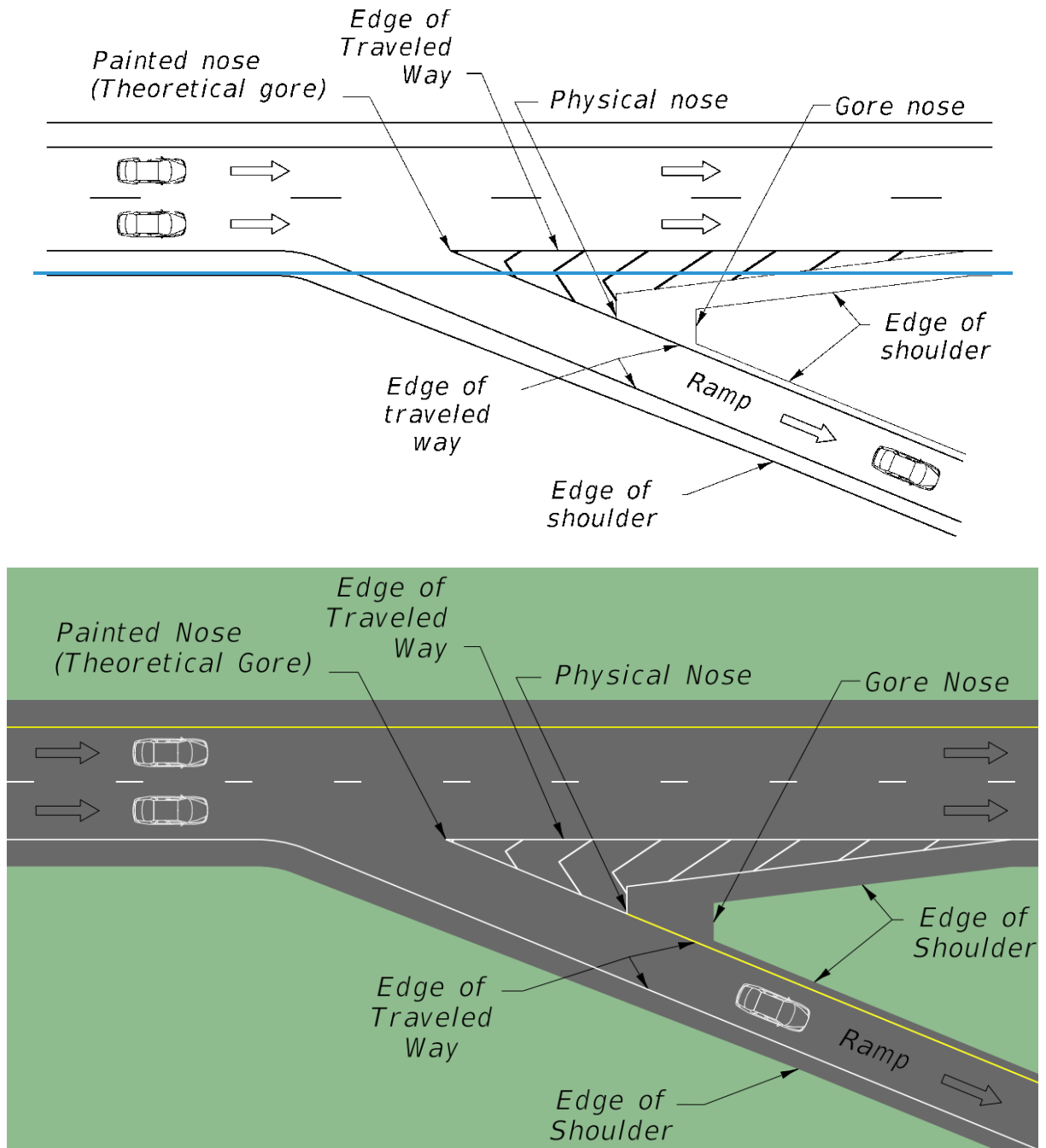
Figure 211.13.1 Ramp Gore
