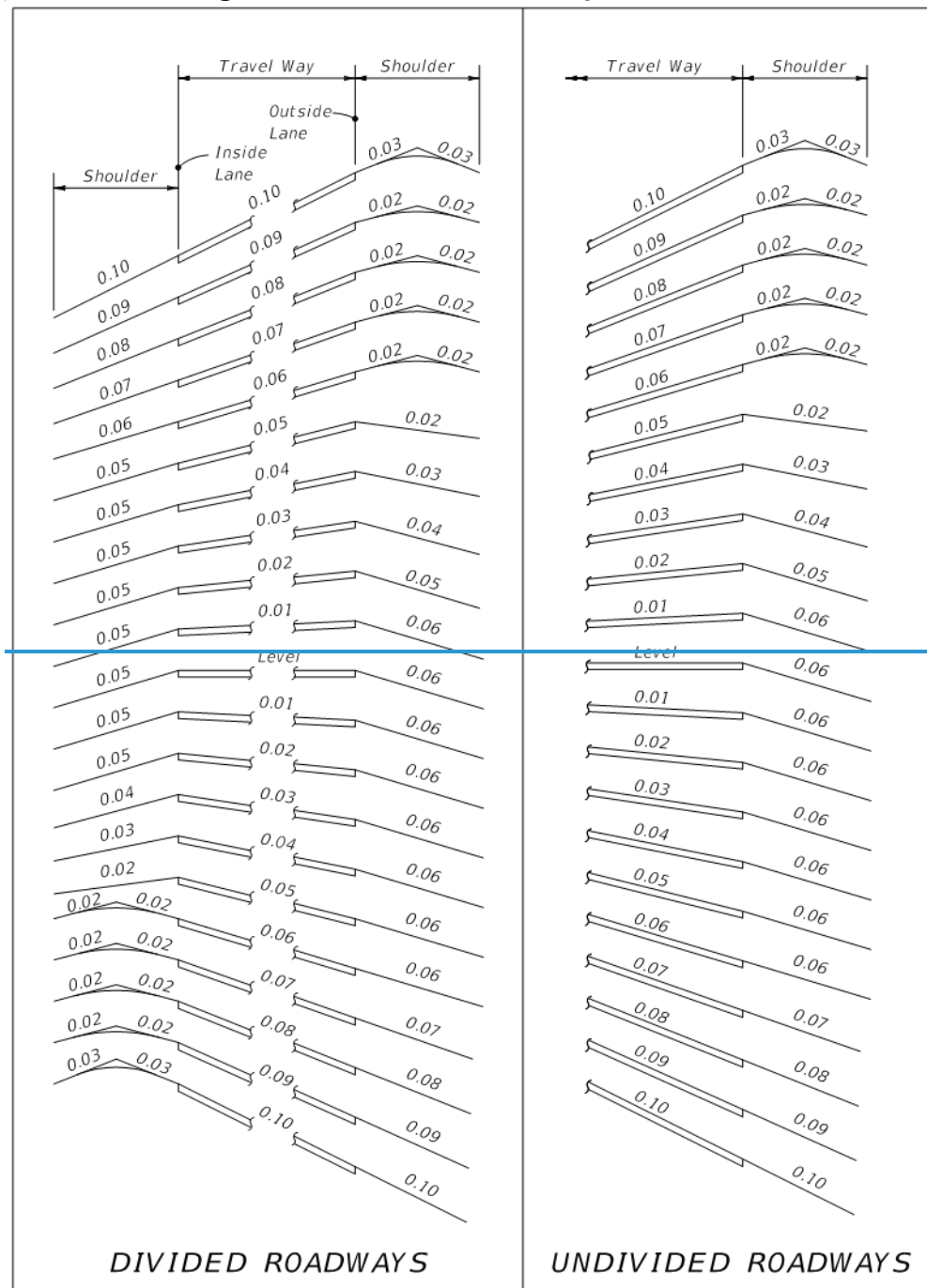
Figure 210.4.2 Shoulder Superelevation
