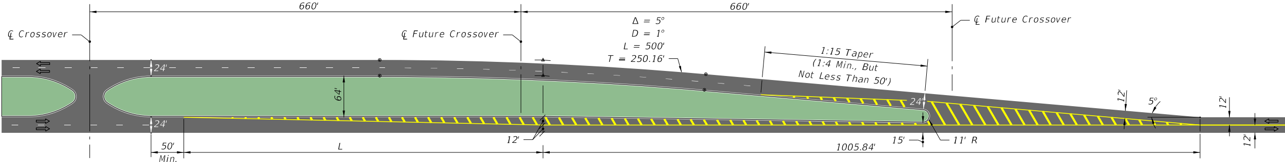
64' MEDIAN
