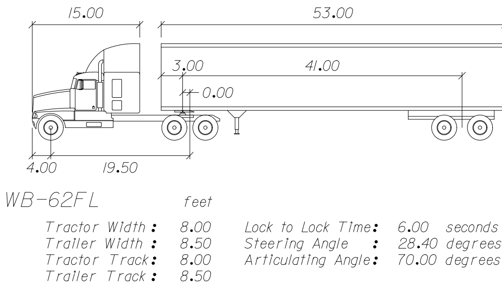
Figure 201.6.1 WB-62FL
