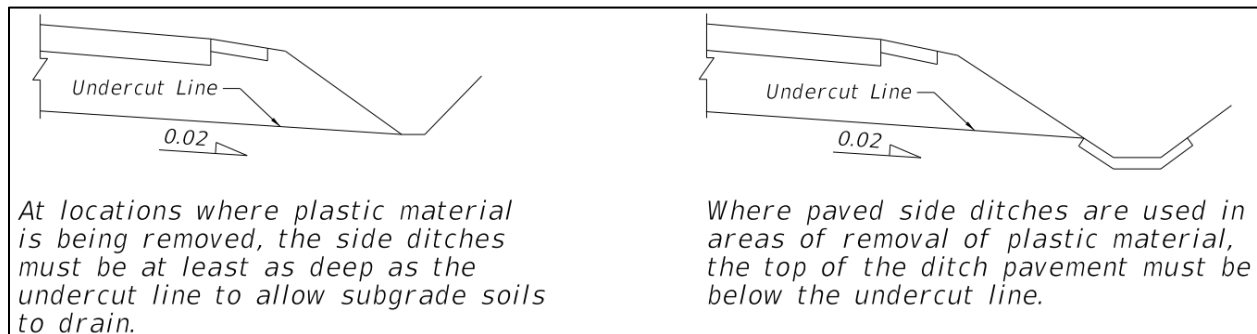
Figure 216.4.7 Undercut Detail of Plastic Material with Relation to Side Ditches
