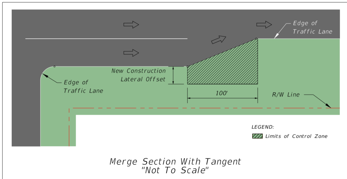
Figure 215.2.8 Merge Section with Tangent
