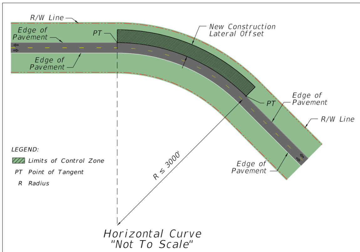
Figure 215.2.12 Horizontal Curve
