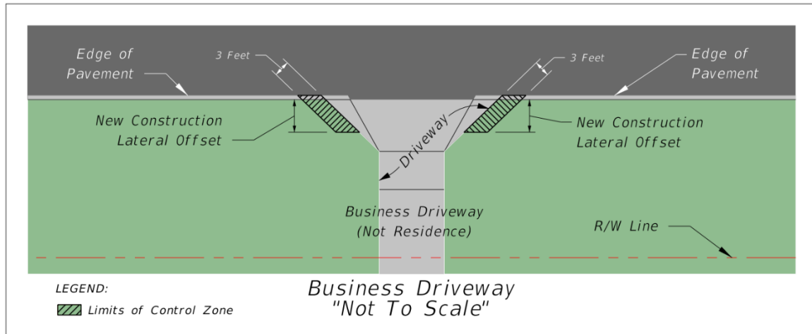
Figure 215.2.11 Business Driveway
