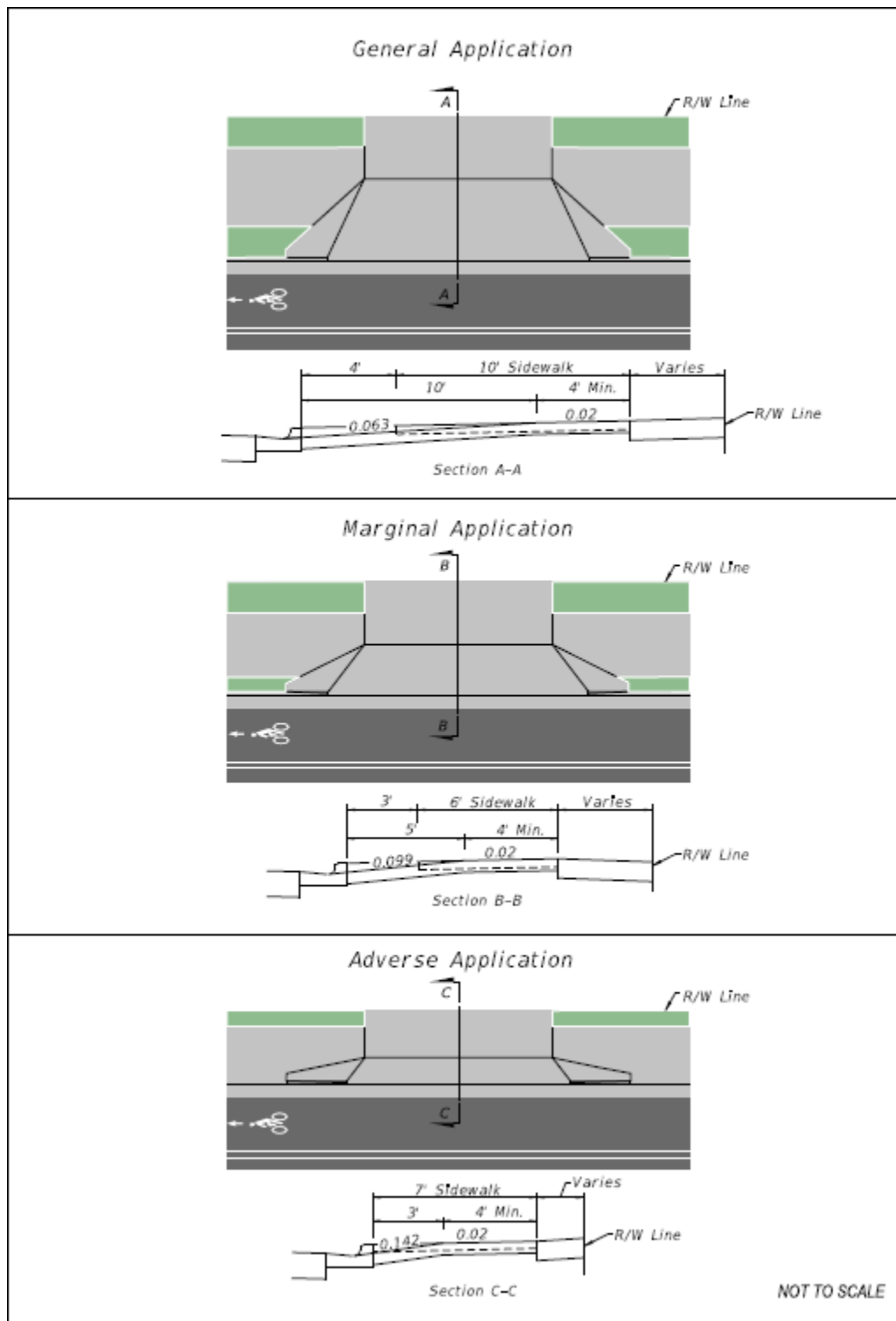
Comparison of Applications for Flared Driveway Connections
