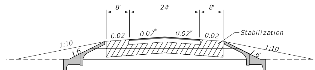
SECTION B-B
