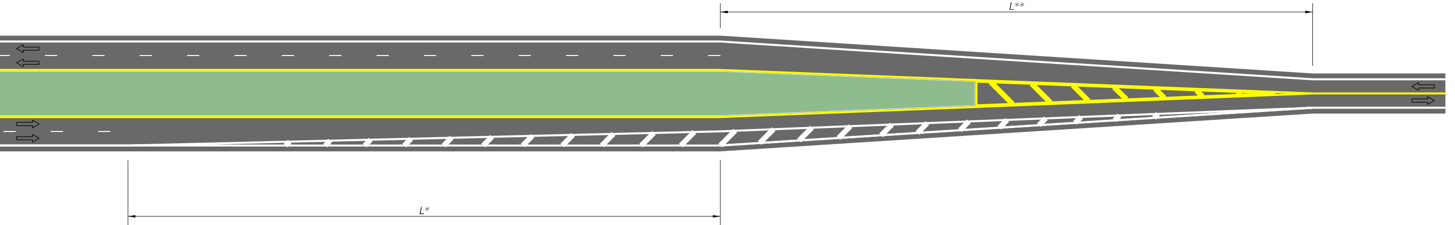
4-LANE DIVIDED TO 2-LANE UNDIVIDED
