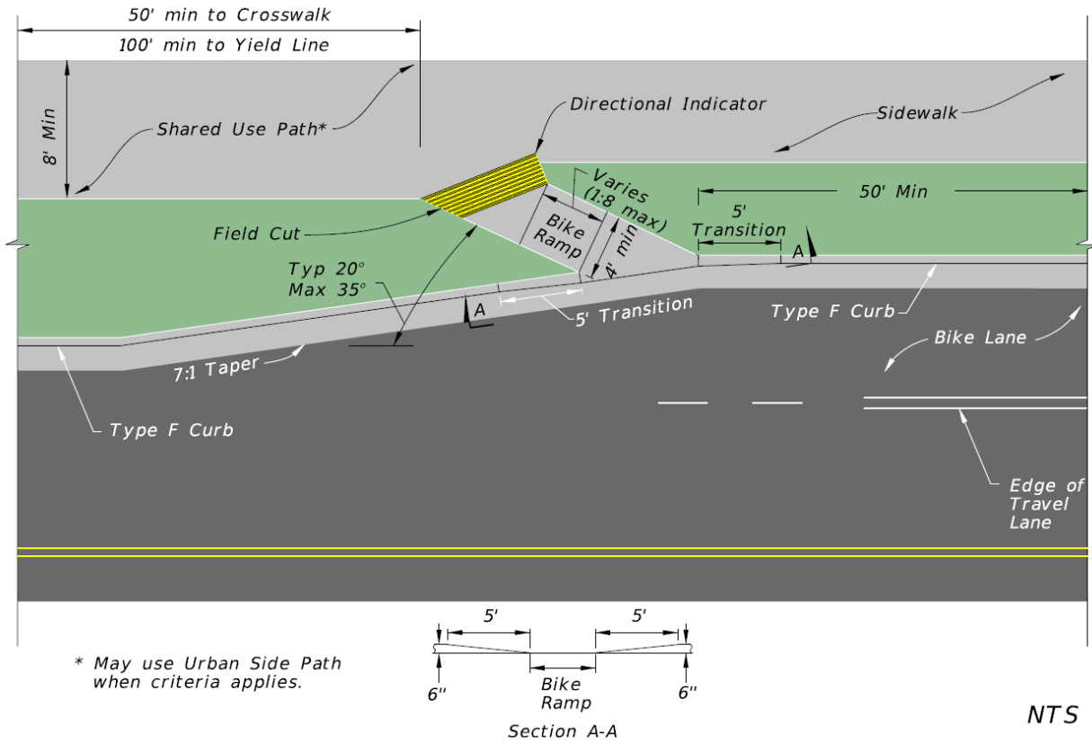
Figure 223.2.5 Angled Bicycle Ramp
