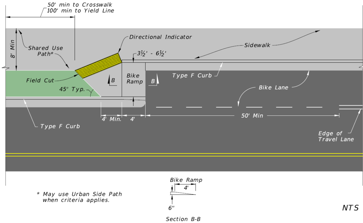
Figure 223.2.6 Straight Bicycle Ramp
