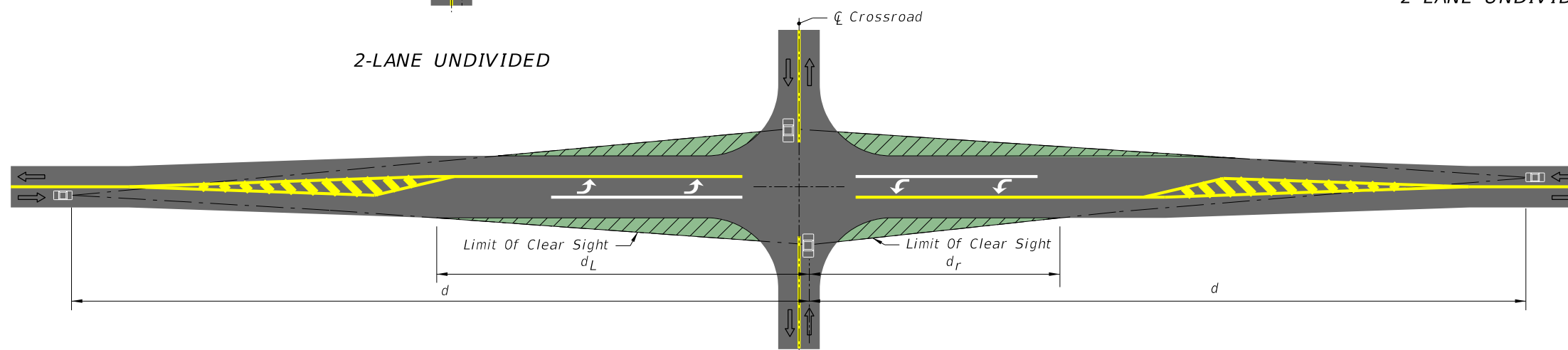
2-LANE WITH LEFT TURN LANE
