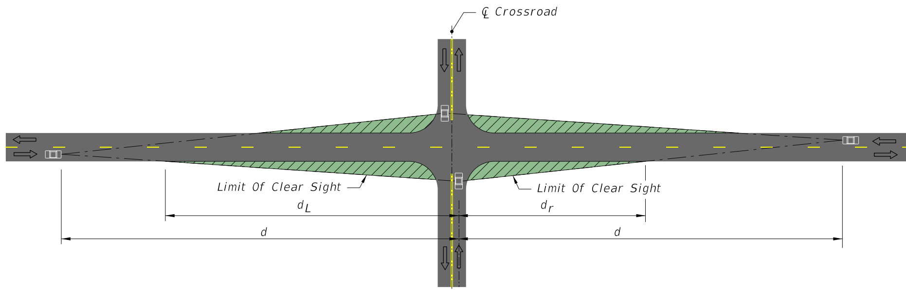
2-LANE UNDIVIDED
