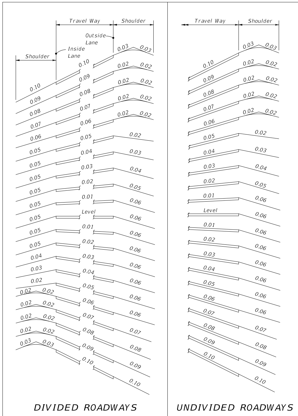
Figure 210.4.2 Shoulder Superelevation
