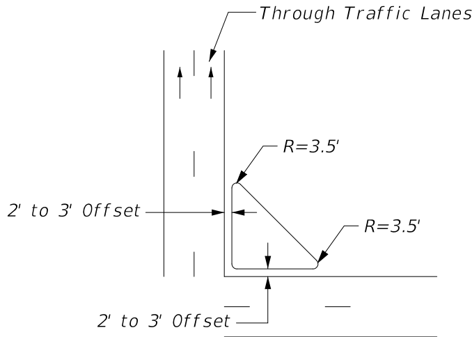
Figure 210.3.1 Typical Small Curbed Island
