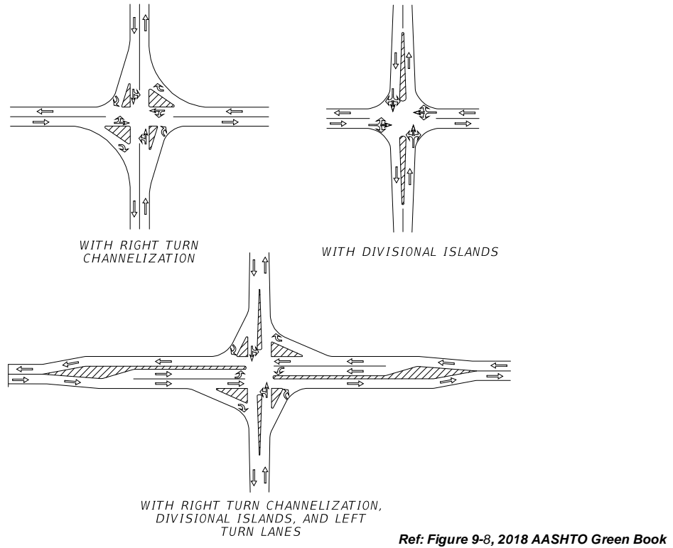
Figure 212.3.2 Channelized Intersections
