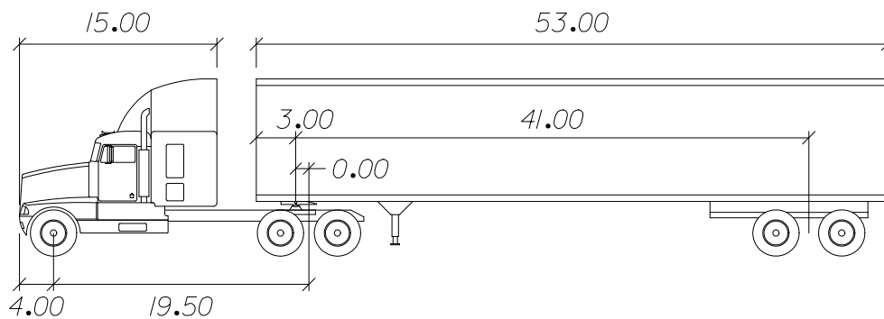
Figure 201.6.1 WB-62FL
