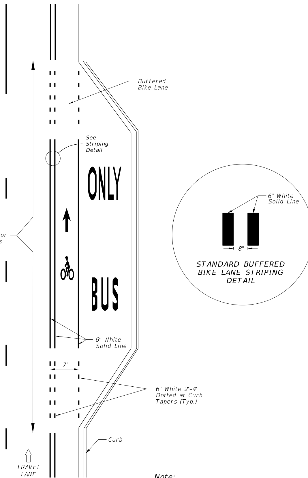
BIKE LANE ADJACENT TO BUS BAY
