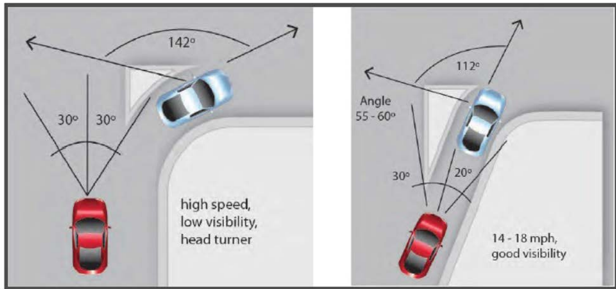
Figure 212.12.2 Channelized Right Turn Lanes
