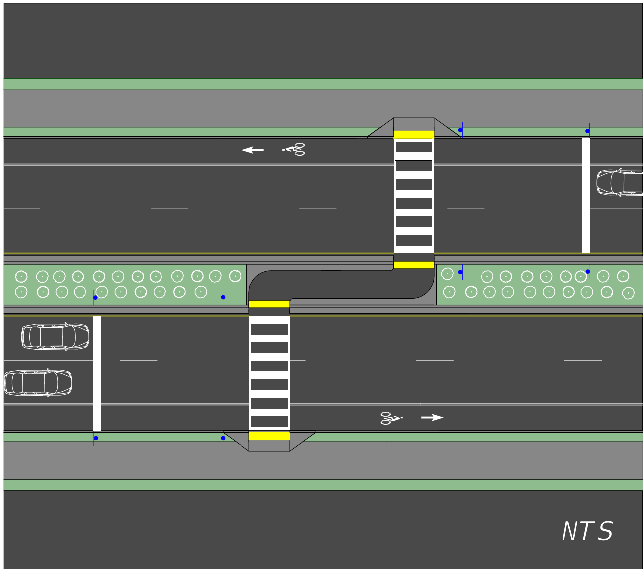
Figure 212.13.4 Pedestrian Refuge Island Example #2
