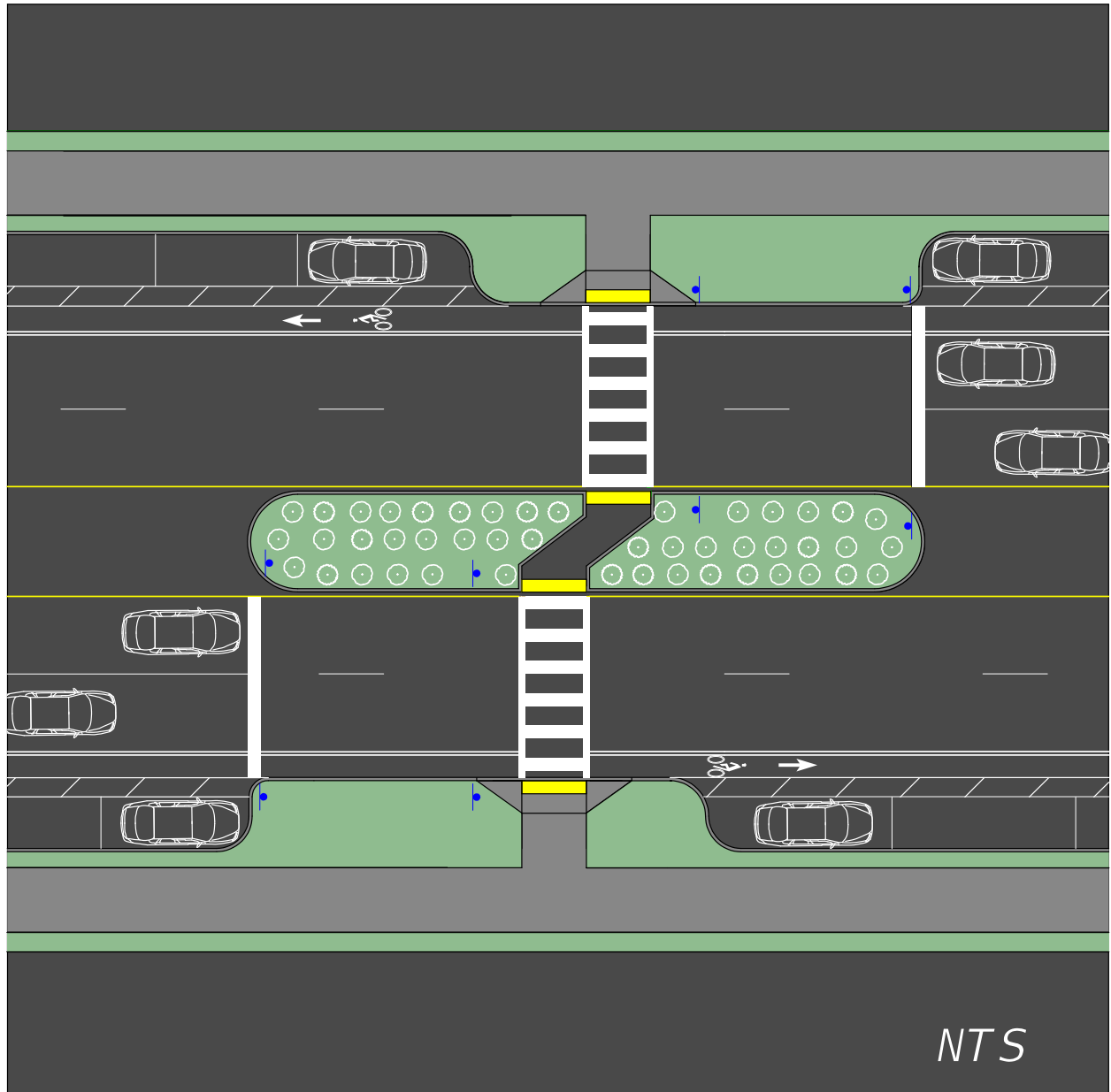
Figure 212.13.3 Pedestrian Refuge Island Example #1
