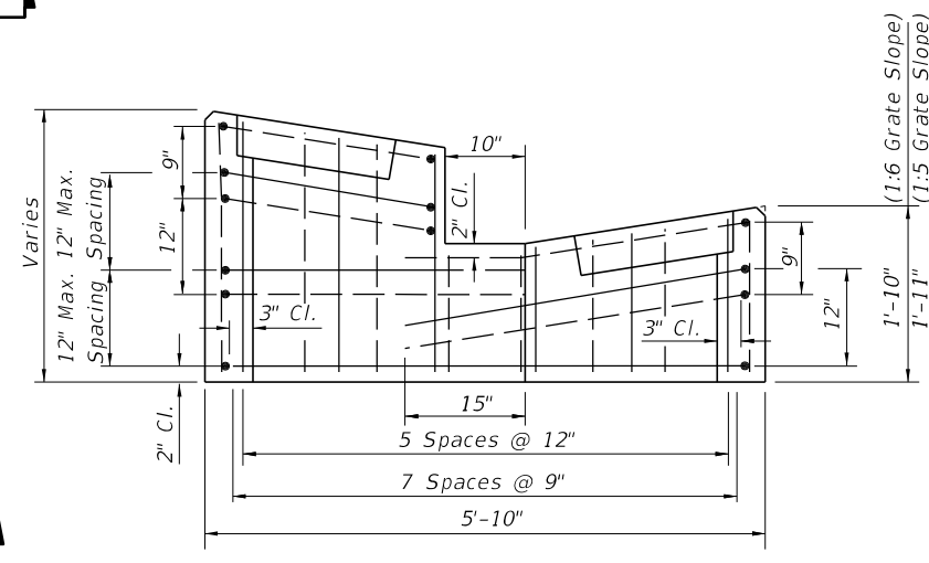
SECTION HH
