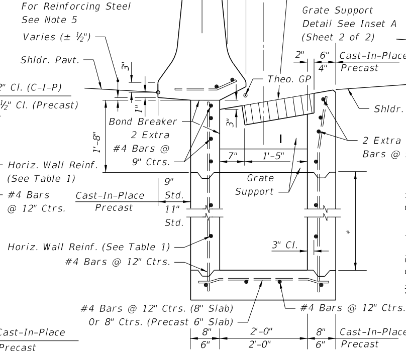
SECTION FOR INLETS TYPES 1 & 2 (Pipe Opening Shown) SECTION BB
