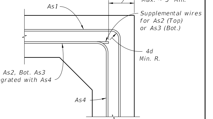
DETAIL "A" (OPTION 3)
