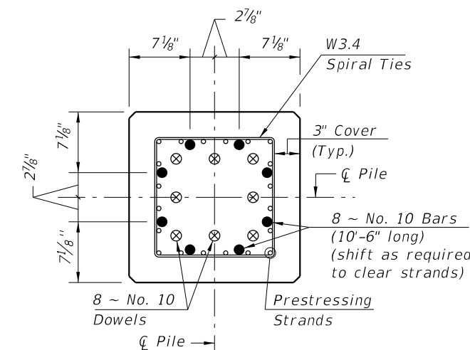
SECTION F-F
