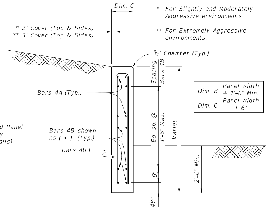
SECTION C-C
