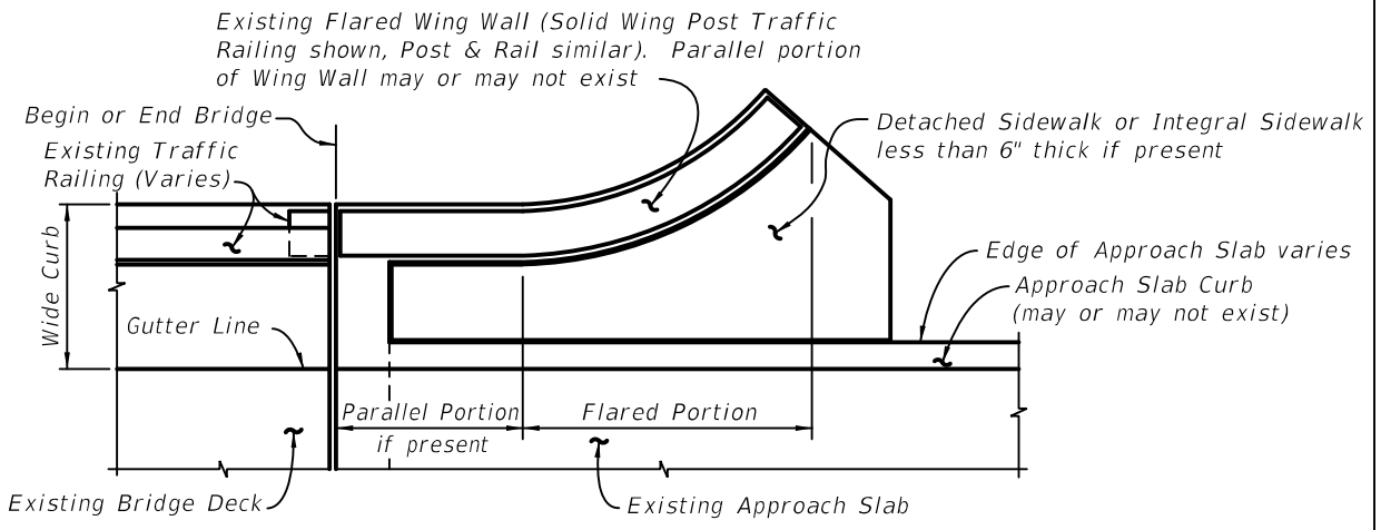
PARTIAL PLAN VIEW OF EXISTING BRIDGE WITH WIDE CURBS, FLARED WING WALLS AND APPROACH SLABS WITH DETACHED SIDEWALKS OR SIDEWALKS LESS THAN 6" THICK - USE INDEX NO. 482, SCHEME 5
