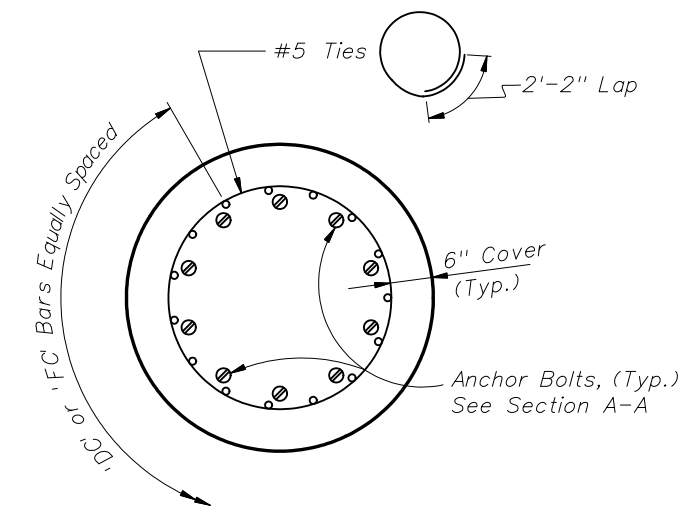
PLAN VIEW DRILLED SHAFT
