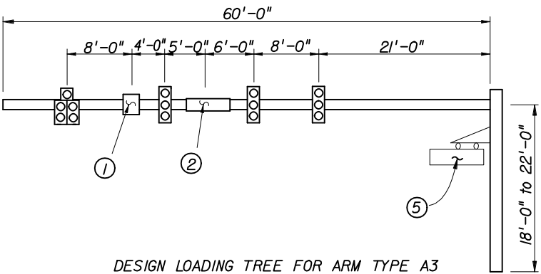
DESIGN LOADING TREE FOR ARM TYPE A3
