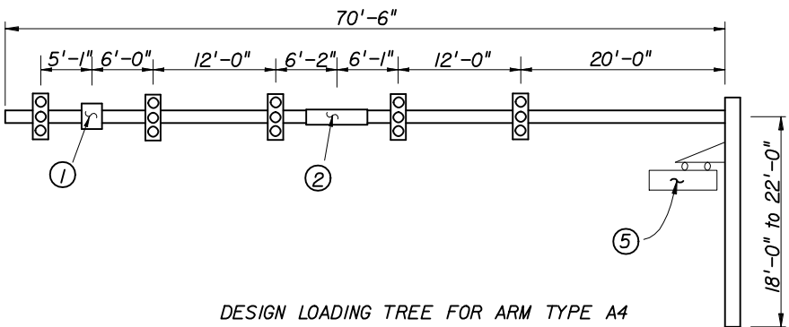
DESIGN LOADING TREE FOR ARM TYPE A4
