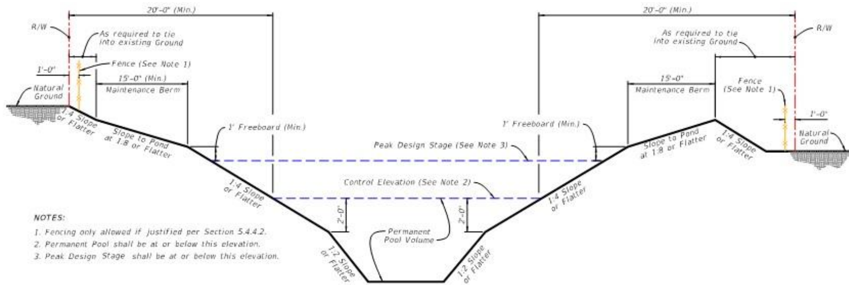
Figure 5-2: Minimum Clearance for Stormwater Management Facilities
