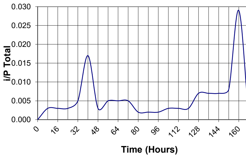
7 Day Duration Intensity Curve
