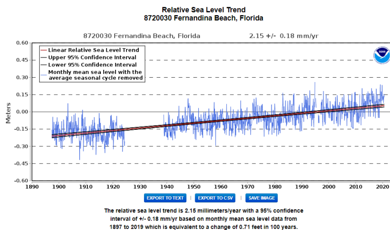
Figure 3-1: Relative Sea Level Trend Data Example
