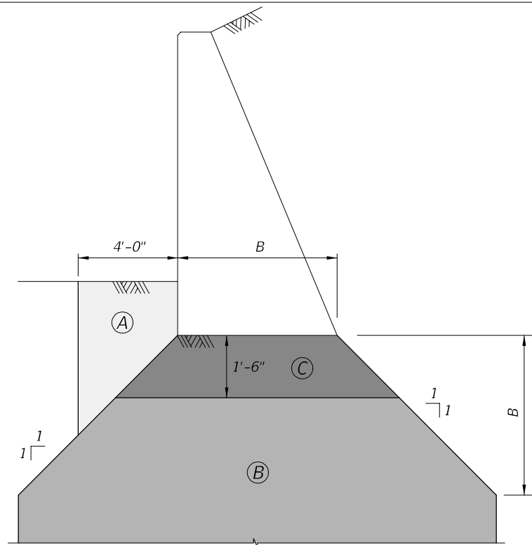
SECTION THRU CAST IN PLACE GRAVITY WALL (INDEX 400-011)
