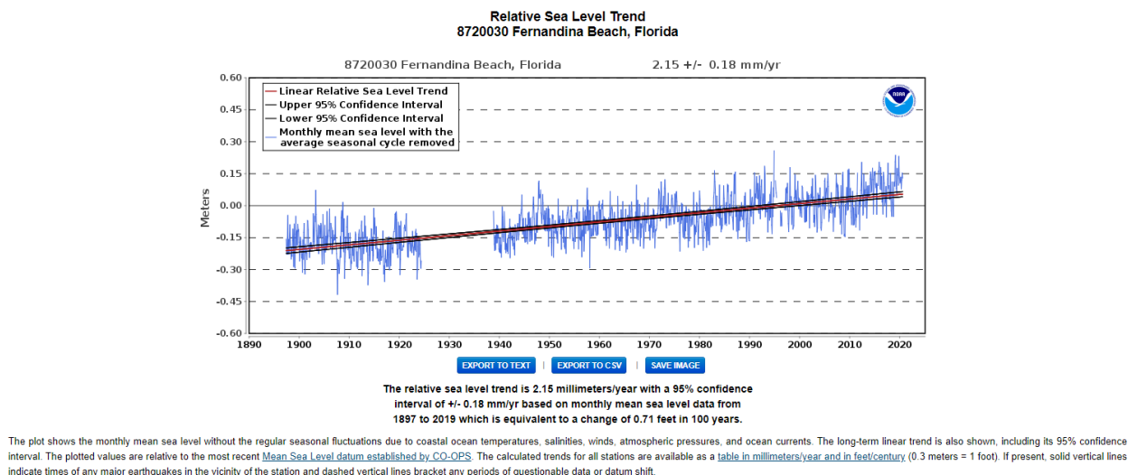
Figure 3-1: Relative Sea Level Trend Data Example
