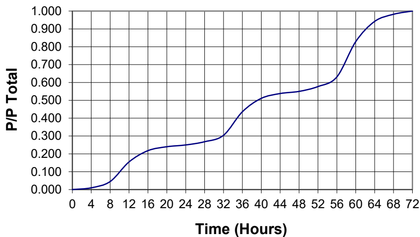
3 Day Duration Mass Rainfall Curve
