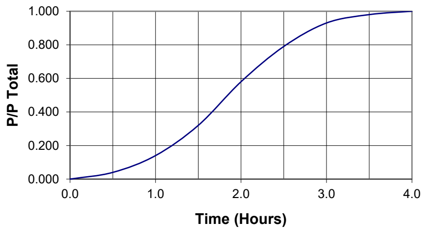
4 Hour Duration Mass Rainfall Curve
