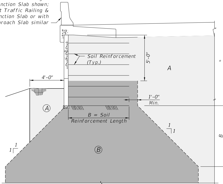
SECTION THRU PERMANENT MSE WALL* (INDEX 548-020)
