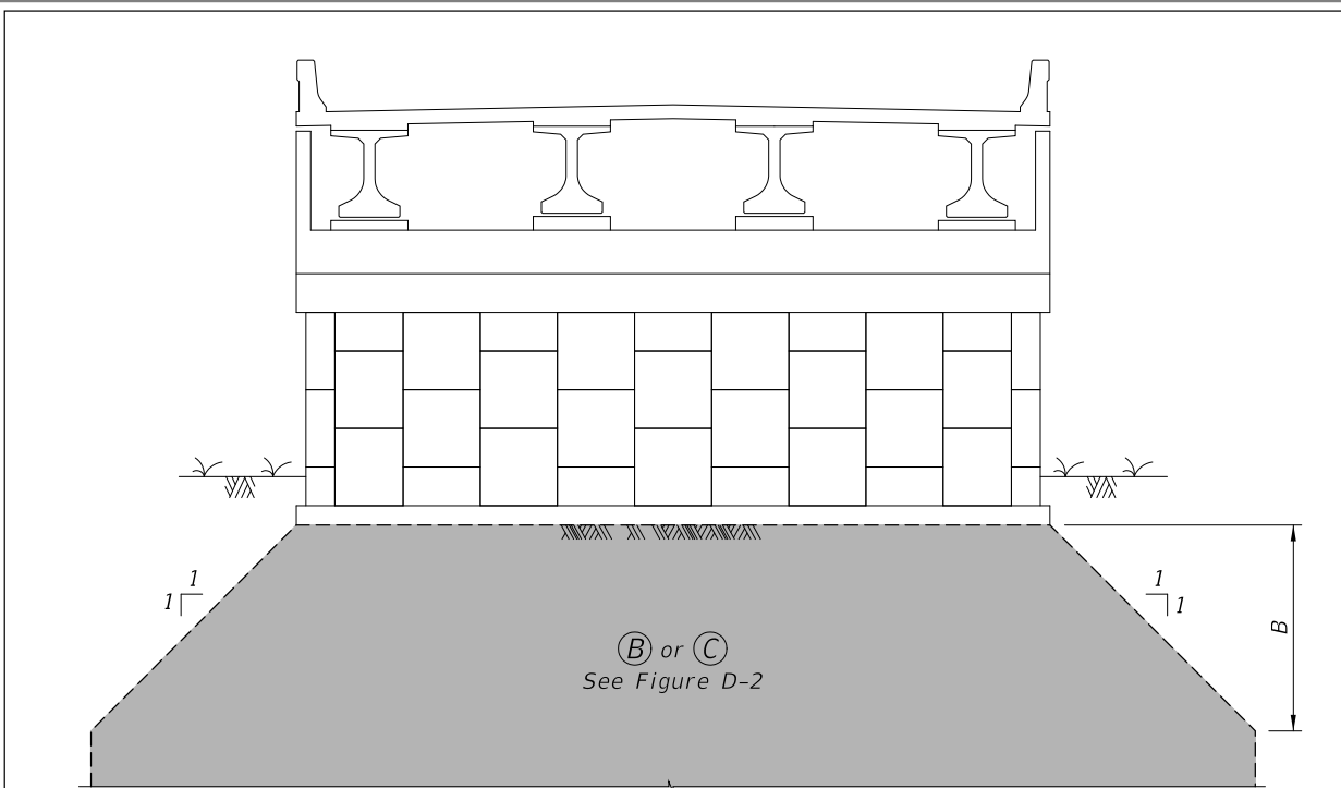
ELEVATION VIEW - PERMANENT MSE WALL* W/ BRIDGE ABUTMENT ON DEEP OR SHALLOW FOUNDATION (INDEX 548-020)
