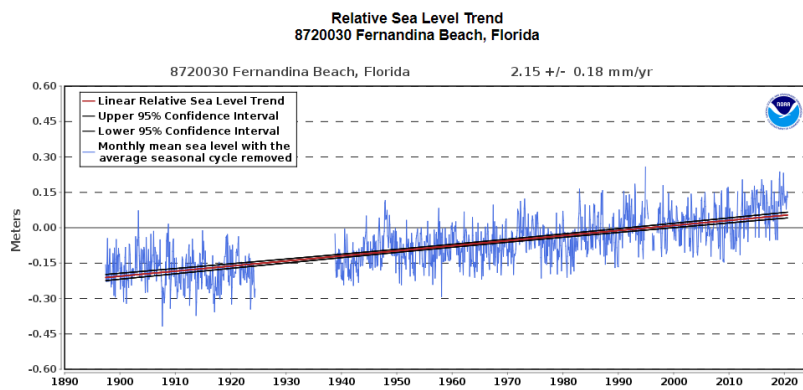
The relative sea level trend is 2.15 millimeters/year with a 95% confidence interval of +/- 0.18 mm/yr based on monthly mean sea level data from 1897 to 2019 which is equivalent to a change of 0.71 feet in 100 years.
